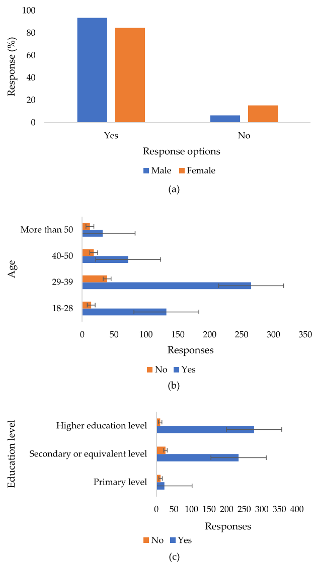
Fig. 2 Purchase of preserved food declaration (a) based on gender (b) based on age (c) based on educational level
