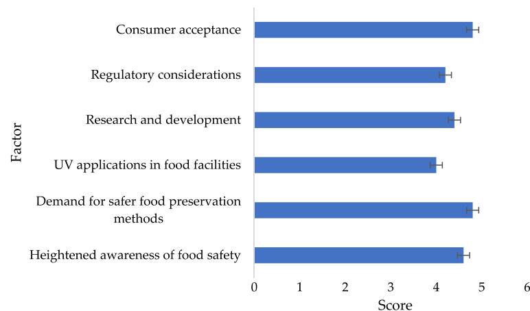
Fig. 4 COVID-19 potential influence on the adoption of UV irradiation for preservation of fruits and vegetables
