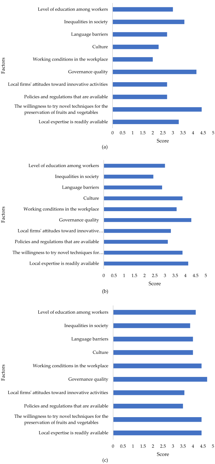
Fig. 5 Score of social factors affecting innovation in the fruits and vegetables preservation sector (a) small scale (b) medium scale (c) large scale
