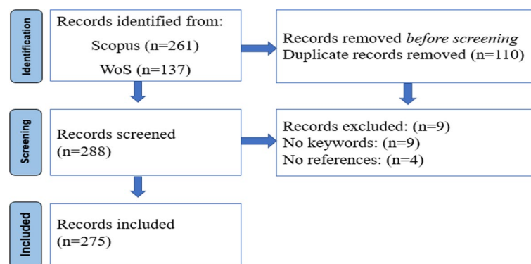
Fig. 1 PRISMA flowchart
