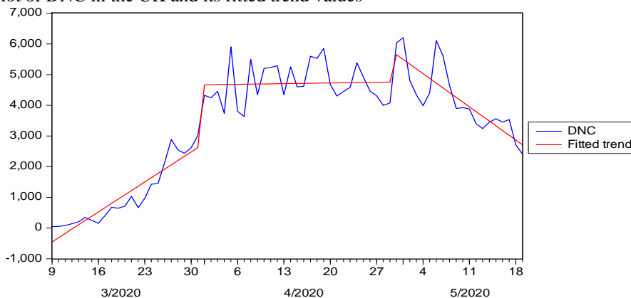
Figure 4.16 Plot of DNC in the UK and its fitted trend values
