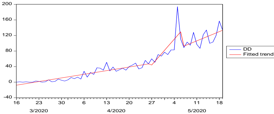
Figure 4.18 Plot of DD of India and the fitted trend values
