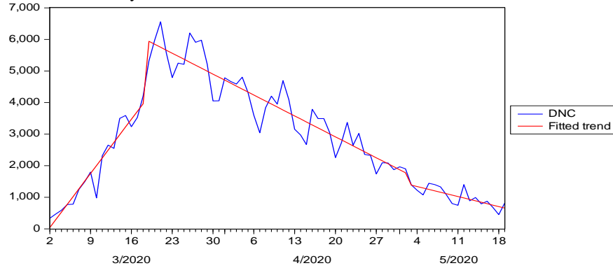
Figure 4.15 Plot of DNC in Italy and its fitted trend values
