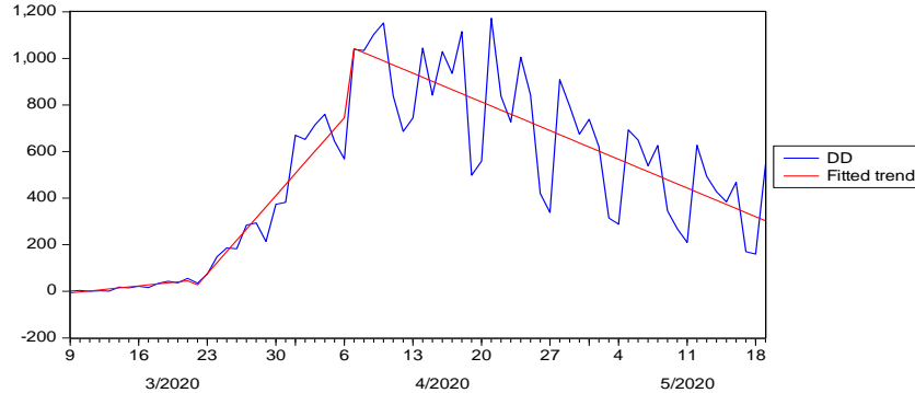
Figure 4.20 Plot of DD of the UK and the fitted trend values
