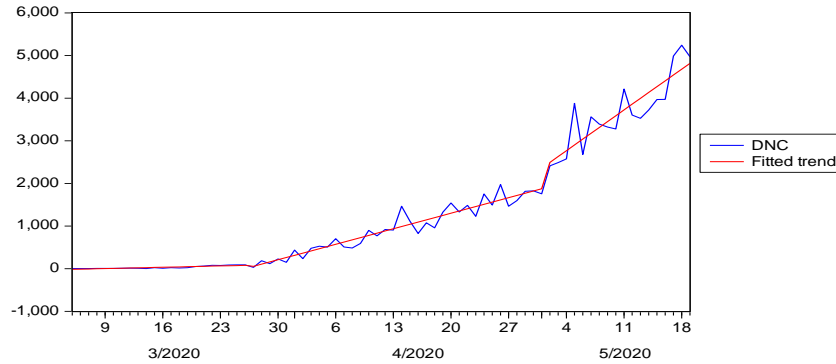
Figure 4.14 Plot of DNC in India and its fitted trend values
