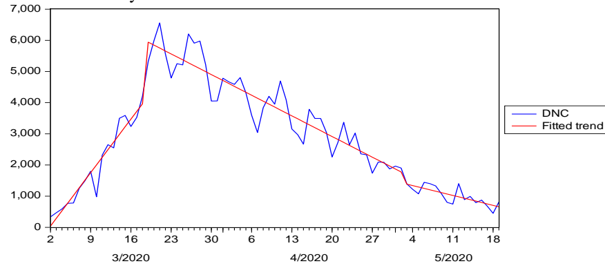
Figure 4.15 Plot of DNC in Italy and its fitted trend values
