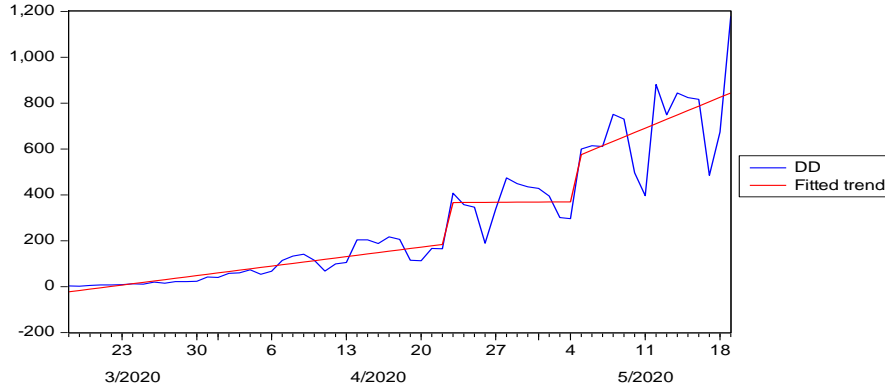
Figure 4.17 Plot of DD of Brazil and the fitted trend values
