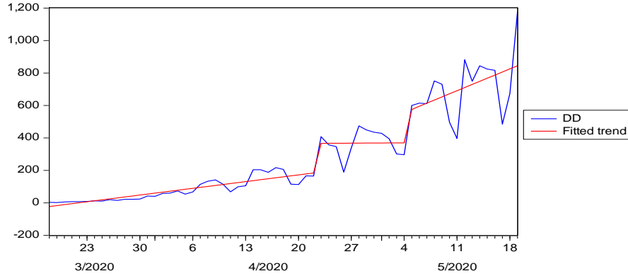
Figure 4.18 Plot of DD of India and the fitted trend values
