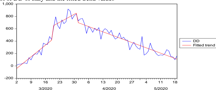
Figure 4.19 Plot of DD of Italy and the fitted trend values
