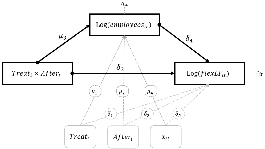
Figure 3: Mediation model
