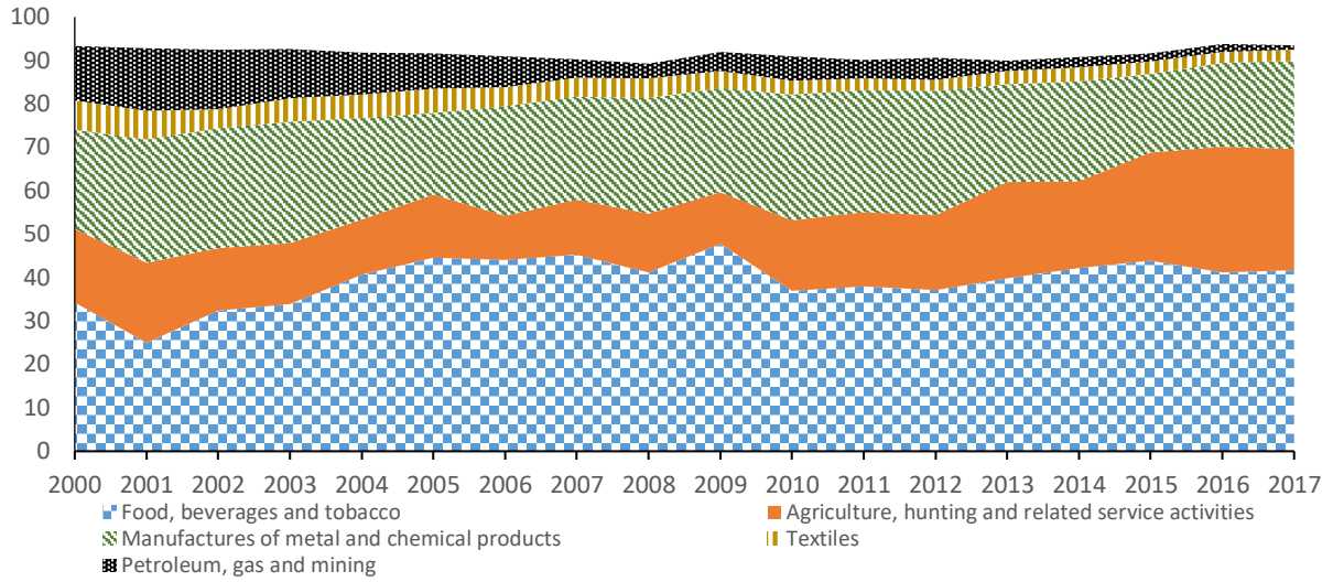
Figure 4.5. Emissions: Main Contributing Sectors
