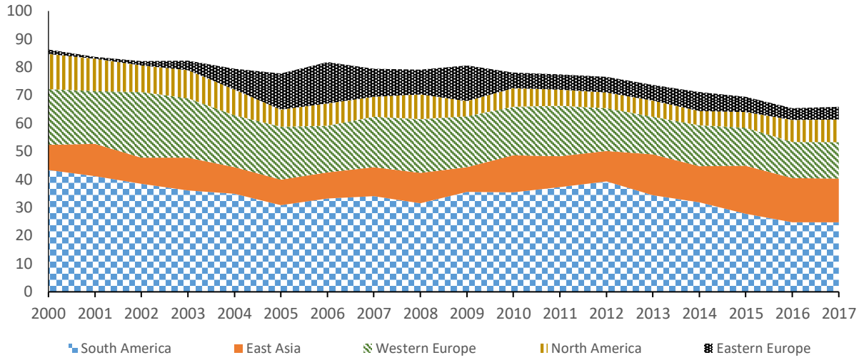
Figure 4.6. Emissions: Main Contributing Partners
