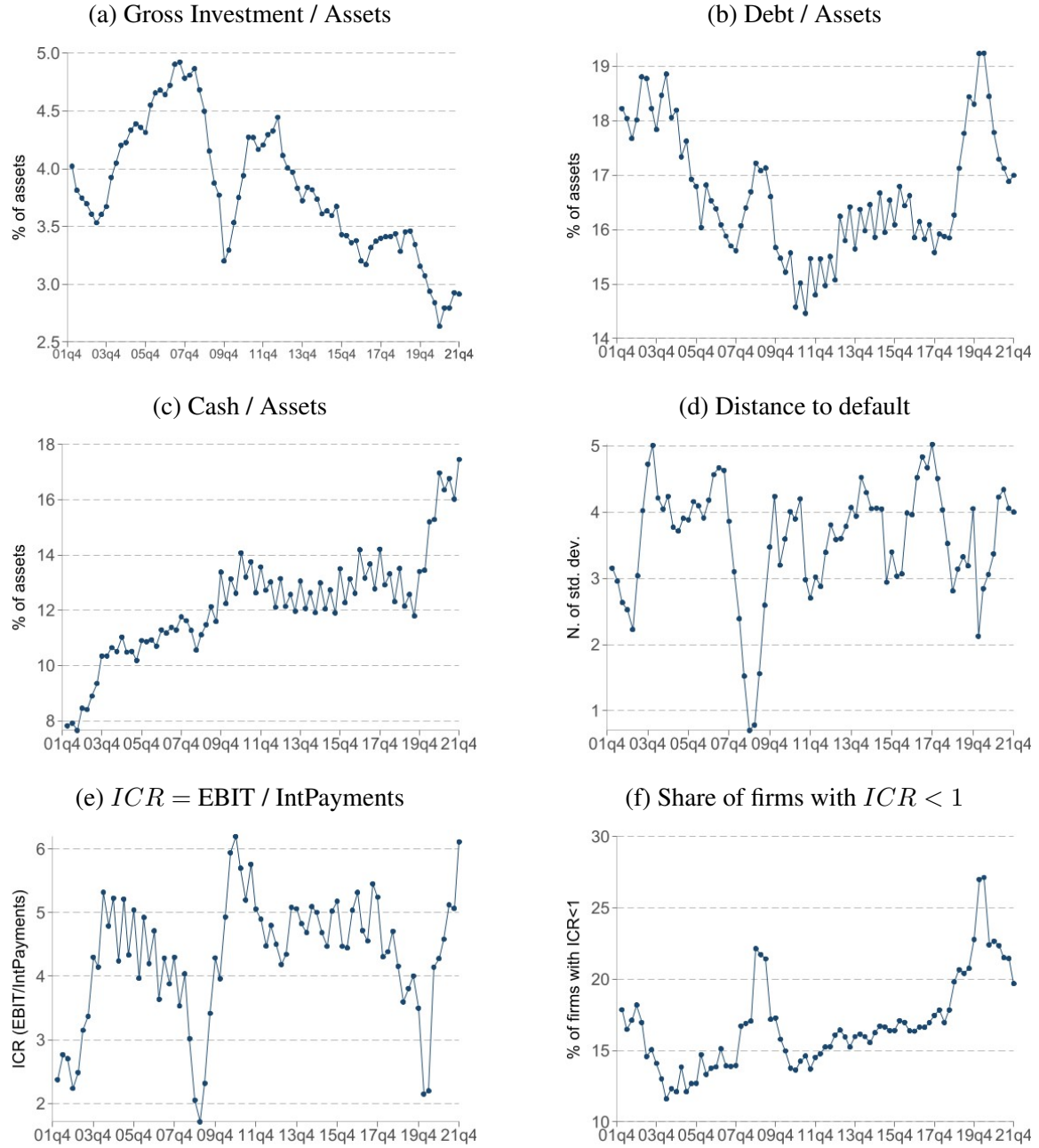
Figure 2: Evolution of Key Variables (medians)
