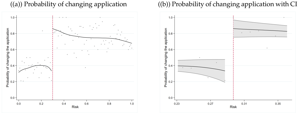
Figure 1: RDD results on application changes during the validation period
