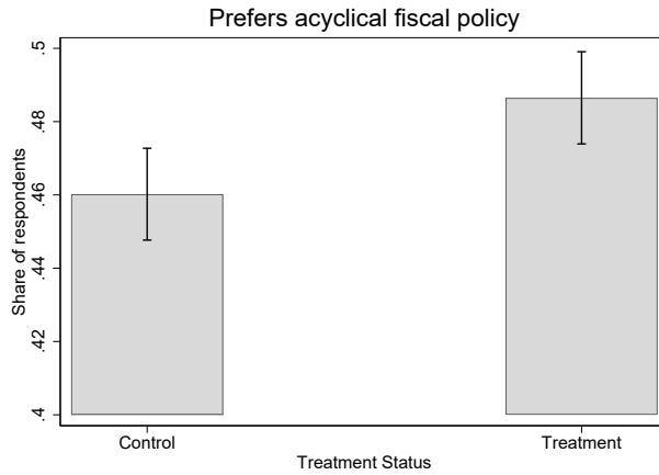
(a) Acyclical
