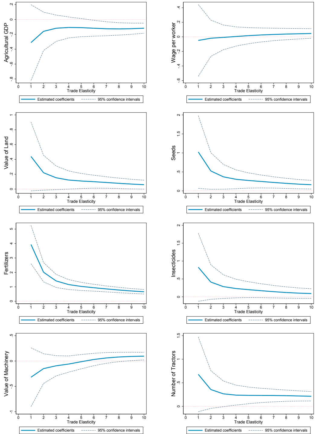
FIGURE A.5.1 BETA COEFFICIENTS FOR DIFFERENT TRADE ELASTICITIES-OLS
