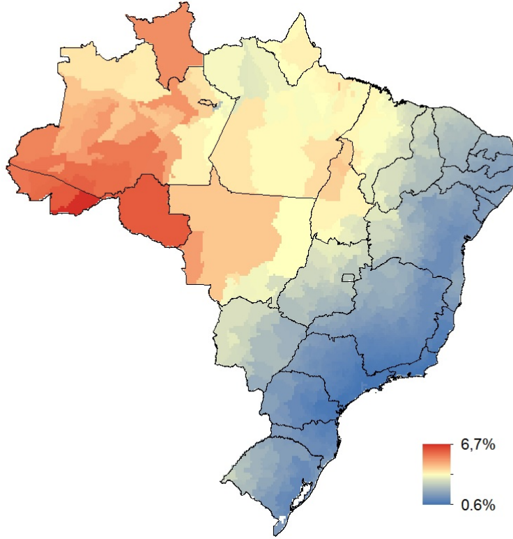
FIGURE 3 YEARLY GROWTH RATE OF MARKET ACCESS:1950–2000
