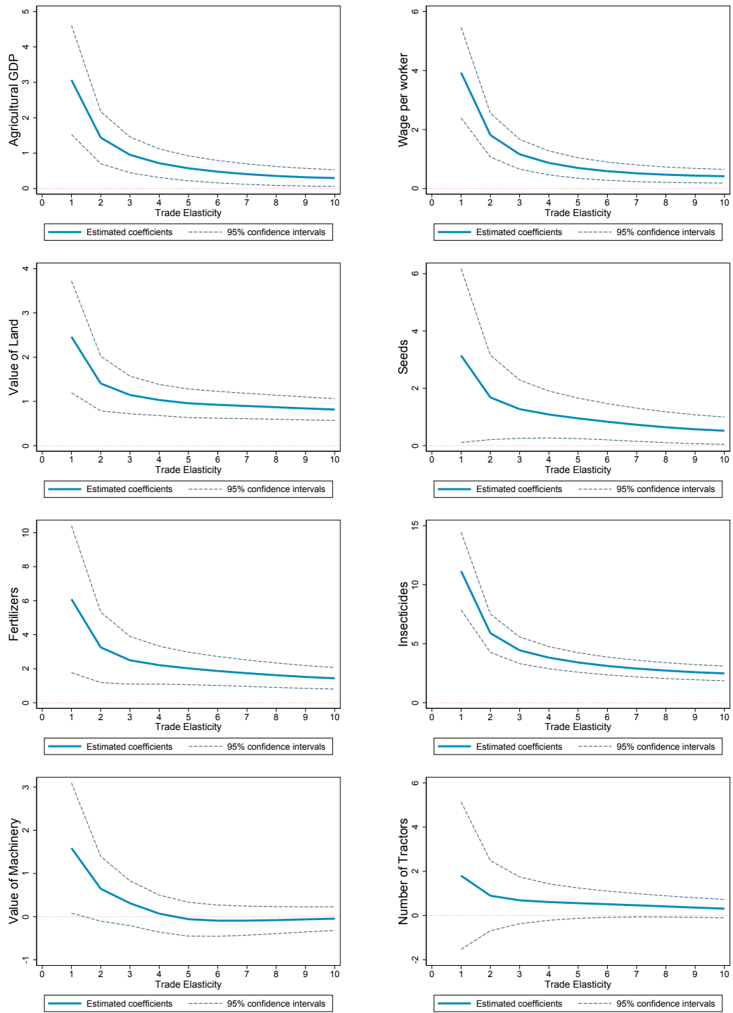
FIGURE A.5.2 BETA COEFFICIENTS FOR DIFFERENT TRADE ELASTICITIES-IV
