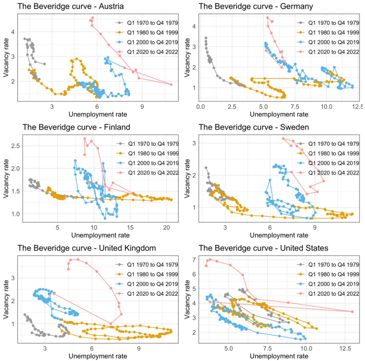
Figure 2 / Beveridge curve, 1970-2022
