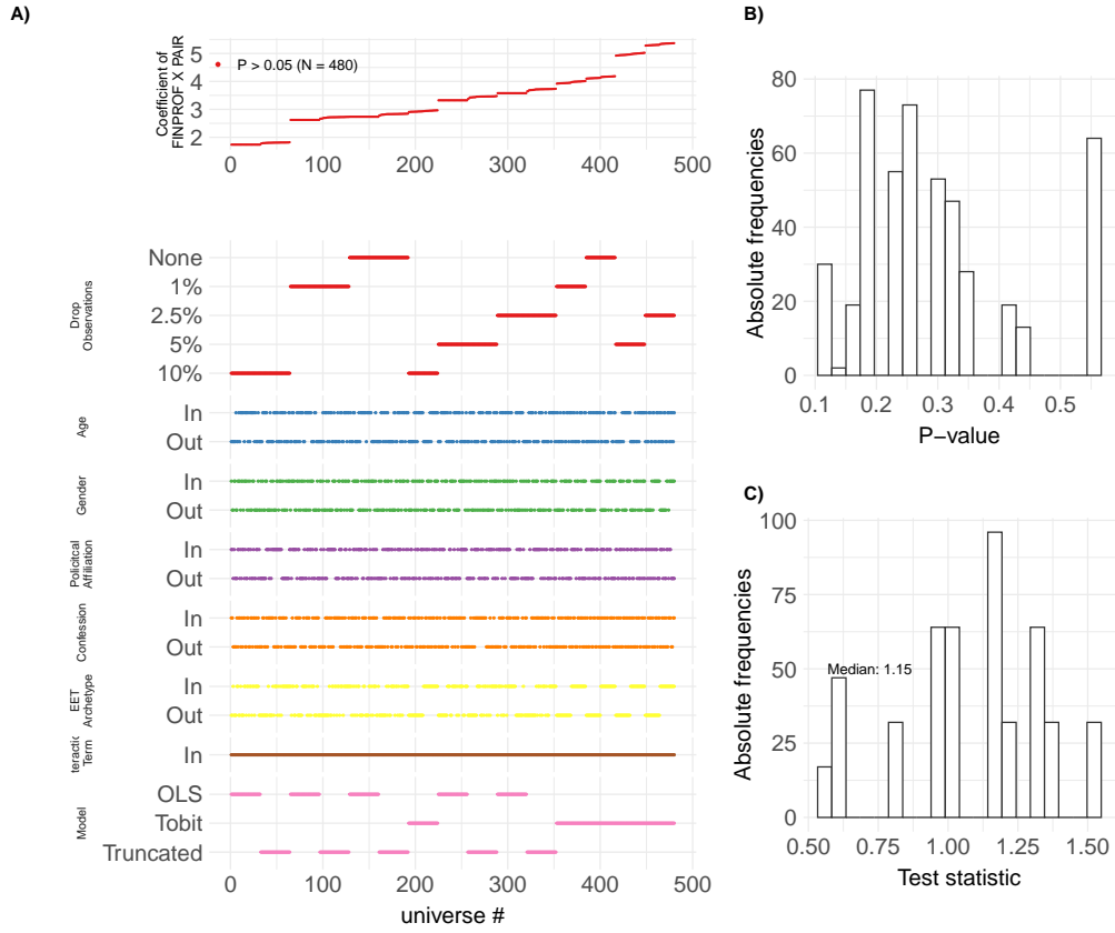
Figure A1: Specification curve Analysis for FINPROF \times PAIR . This figure illustrates the results of the specification curve analysis for the interaction between the dummies FINPROF and PAIR , i.e., comparing students' individual decision and professionals' decisions in teams. On top of A) the distribution of coefficients is shown with significance indicator color coded (red = P \geq 0.05 and non significant). None out of 580 specifications yield significant coefficients for making the decision in a pair of financial professionals. Below indicators for specifications within the forks are shown. In Panel B) the distribution of P-values is depicted. In C) the distribution of test statistics (i.e., t-statistic for OLS and Tobit regressions, z-statistic for truncated regression) is shown. The overall median test statistic across all universe is 1.01.
