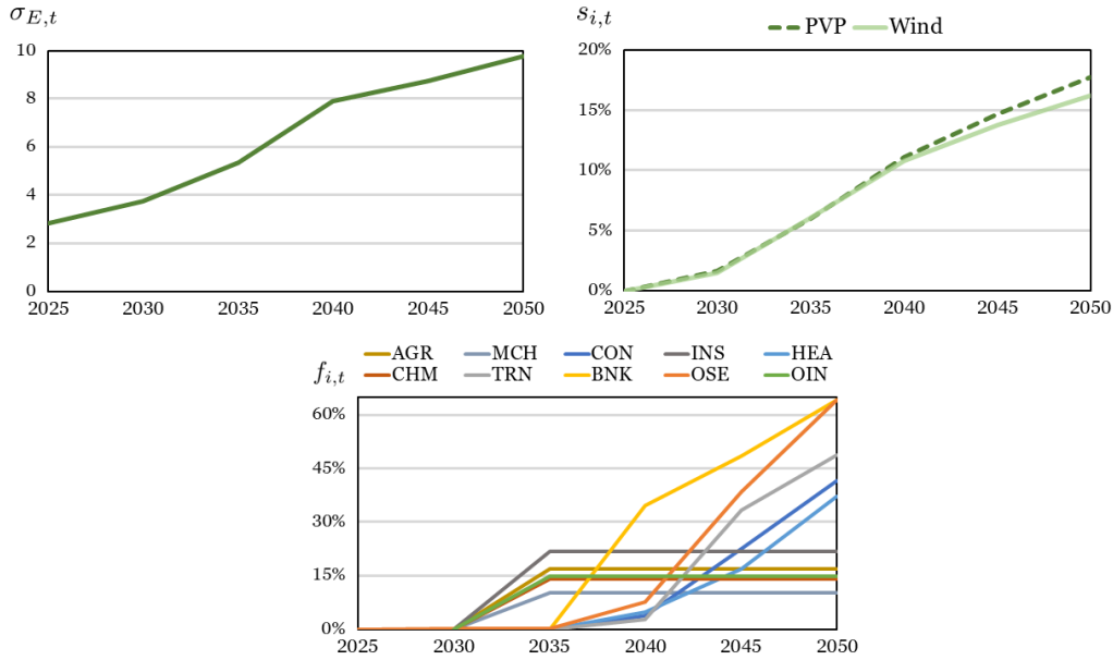
Figure A.5: Evolution of the elasticity of substitution ( \sigma_{E,t} ), the learning factors ( s_{i,t} ) and the energy efficiency improvements ( f_{i,t} ) in the case of the net-zero target when all three feedback mechanisms are in place.
