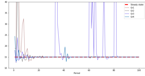
(b) \lambda = 3.5
