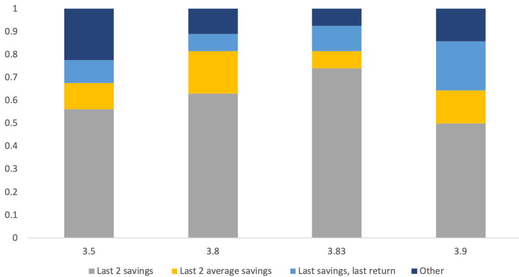
Figure 4.12: Composition of decision rules by treatment (108 subjects)
