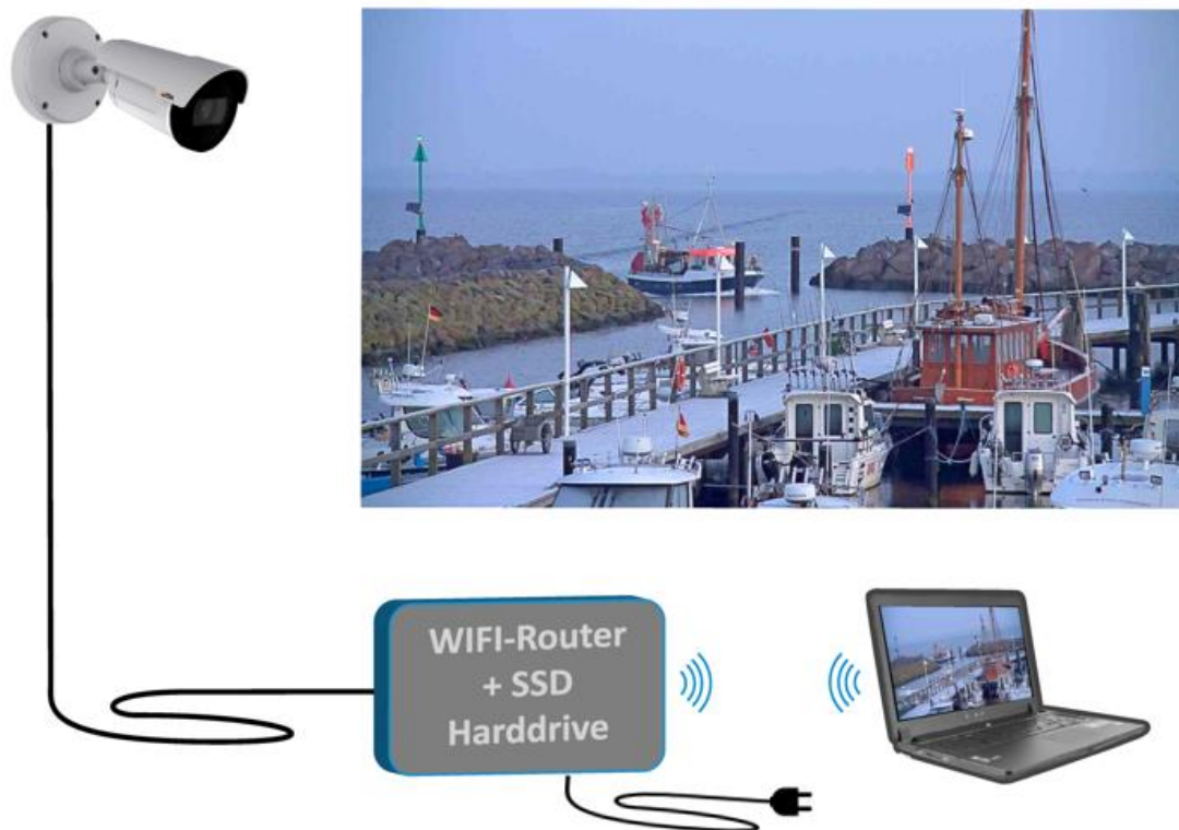
Fig. 9: Setup of the remote camera systems used to monitor the recreational salmon trolling effort around the Island of Rügen.
