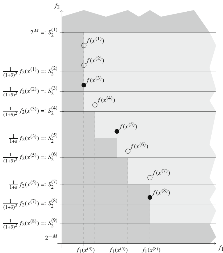
Fig. 4 An illustration of Algorithm 2 in the objective space (on a logarithmic scale). Each x^{(i)} is a solution to \text{DUALRESTRICT}_\delta^1(S_2^{(i)}) for i = 1, \dots, 8 , where (1 + \delta)^4 = (1 + \varepsilon) . The dark gray region does not contain any feasible point. Any feasible point in the light gray region is (1, 1 + \varepsilon) -dominated by f(x^{(i)}) for some i \in \{1, \dots, 8\} . The solution x^{(4)} is discarded since any solution that is (1, 1 + \varepsilon) -approximated by x^{(4)} is also (1, 1 + \varepsilon) -approximated by x^{(3)} or x^{(5)} . The solution x^{(6)} is discarded since any solution that is (1, 1 + \varepsilon) -approximated by x^{(6)} is also (1, 1 + \varepsilon) -approximated by x^{(5)} or x^{(7)} . The solutions x^{(1)}, x^{(2)} , and x^{(7)} are discarded since they are dominated by x^{(2)}, x^{(3)} , and x^{(8)} , respectively. \text{DUALRESTRICT}_\delta^1(S_2^{(9)}) returns NO, so the algorithm returns \{x^{(3)}, x^{(5)}, x^{(8)}\}
