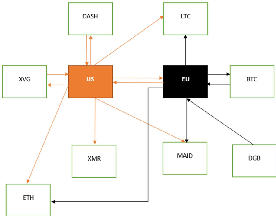
Fig. 6 The causal relationship network between the US and European Crude Oil and Cryptocurrency Markets. Note Three coins have bilateral relationships whereas the remaining coins have a unilateral relationship to a specific crude oil market. The interconnectedness between US and European crude oil markets is one of the key factors enhancing causal relationships among the cryptocurrencies
