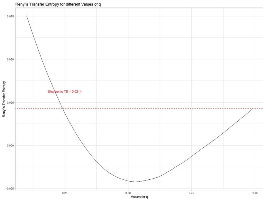
Fig. 5 Rényi transfer entropy with different values of q from the DCOILWTICO to DCOILBRENTU
