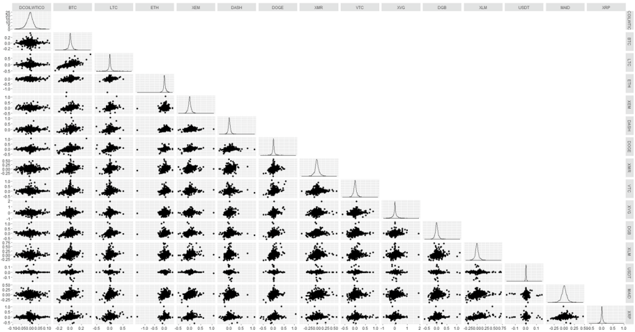
Fig. 1 Data Distribution and Correlation between the US Crude Oil Index and each Cryptocurrency. Note The correlation data have non-normal distribution (not linear). Furthermore, some dataset structures are skewed and heavy-tailed. Interestingly, there are some outliers correlated with the US crude oil index, which means that the dots are at a distance from the sample plot
