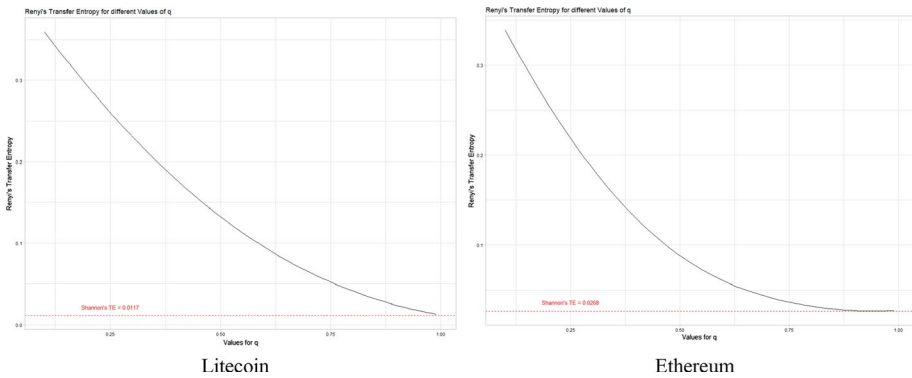
Fig. 3 Rényi transfer entropy with different values of q from the US Crude Oil Market
