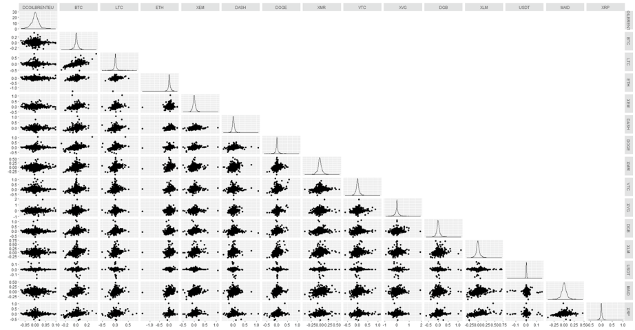
Fig. 2 Data Distribution and Correlation between the European Crude Oil Index and each Cryptocurrency. Note The correlation data have a non-normal distribution (not linear). Furthermore, some dataset structures are skewed and heavy-tailed. Interestingly, there are some outliers correlated with the European crude oil index, which means that the dots are at a distance from the sample plot
