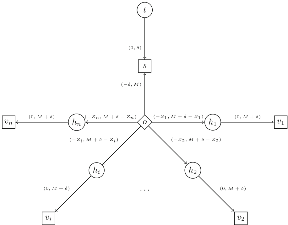
Fig. 1 The graph G(SSP) . Entry nodes are indicated by circles, exits by boxes, and inner nodes by diamonds
