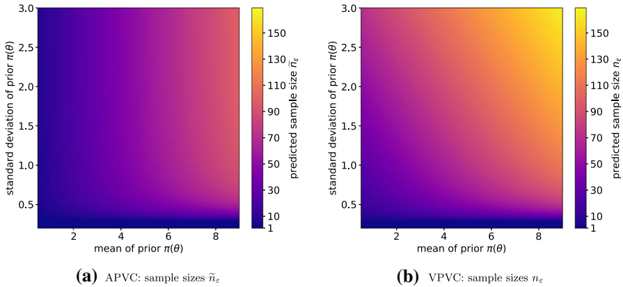
Fig. 2 Left: sample sizes predicted for \text{Poi}(\mathbf{x}_n|\theta) distributed data and various priors \pi(\theta) = \text{Gamma}(\theta|\alpha, \beta) for \varepsilon = 0.3 by the APVC (8). Right: sample sizes n_\varepsilon predicted by the VPVC (9) for the same setup
