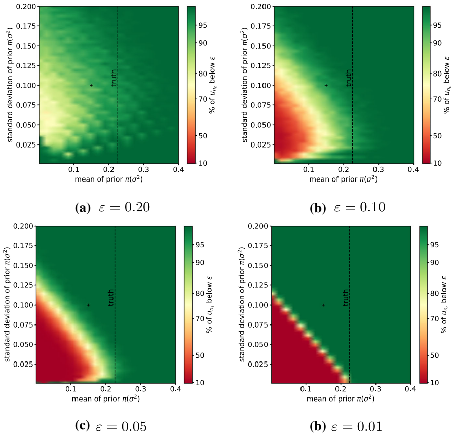
Fig. 8 Percentage of u_{n_\epsilon} < \epsilon for the setup and data from Sect. 2.2 for various \epsilon (in decreasing order), k = 2 , various marginals \pi(\sigma^2) and the same fixed marginal \pi(\mu) as in Fig. 6b. The “true” value of \sigma^2 (computed from the dataset) is depicted by the dashed lines. We used a smaller resolution compared to Fig. 6b for numerical reasons
