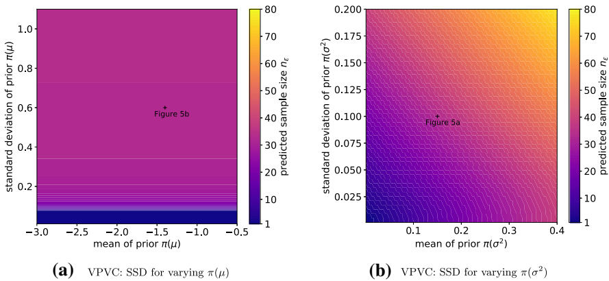
Fig. 5 Sample sizes predicted by the VPVC for different \pi(\mu) and \pi(\sigma^2) . Left: \pi(\sigma^2) is fixed as indicated by the black cross in Fig. 5b and the sample sizes n is depicted for various \pi(\mu) . Right: Sample sizes for various \pi(\sigma^2) and a fixed \pi(\mu) marked by the black cross in Fig. 5a
