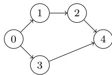
(a) Example activity-on-the-node network
