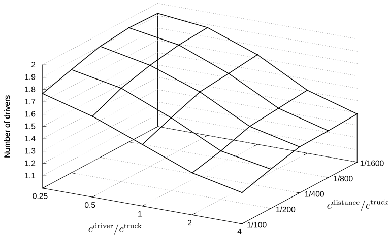
Fig. 17 Average number of drivers for modified Solomon instances for s^{\text{team}} = 0.75 \cdot s^{\text{single}}
