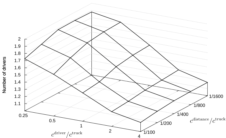
Fig. 18 Average number of drivers for modified Solomon instances for s^{\text{team}} = s^{\text{single}}
