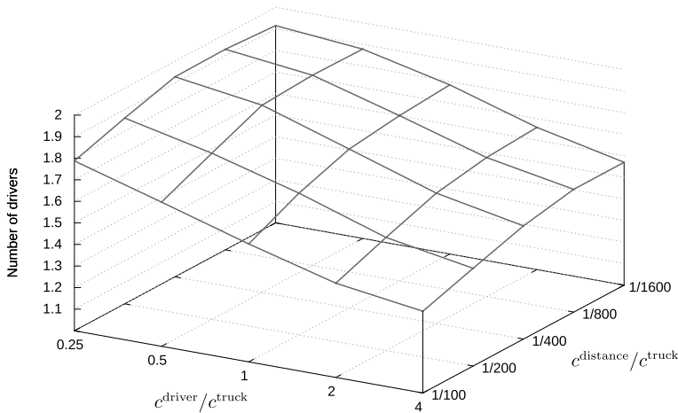
Fig. 16 Average number of drivers for modified Solomon instances for s^{\text{team}} = 0.5 \cdot s^{\text{single}}
