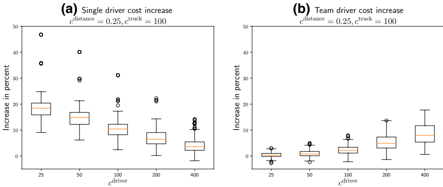
Fig. 14 Cost difference for modified Solomon instances for s^{team} = 0.75 \cdot s^{single}
