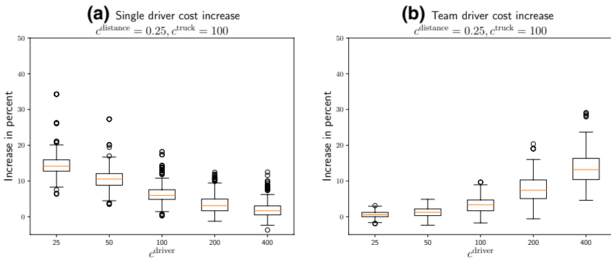
Fig. 15 Cost difference for modified Solomon instances for s^{team} = s^{single}
