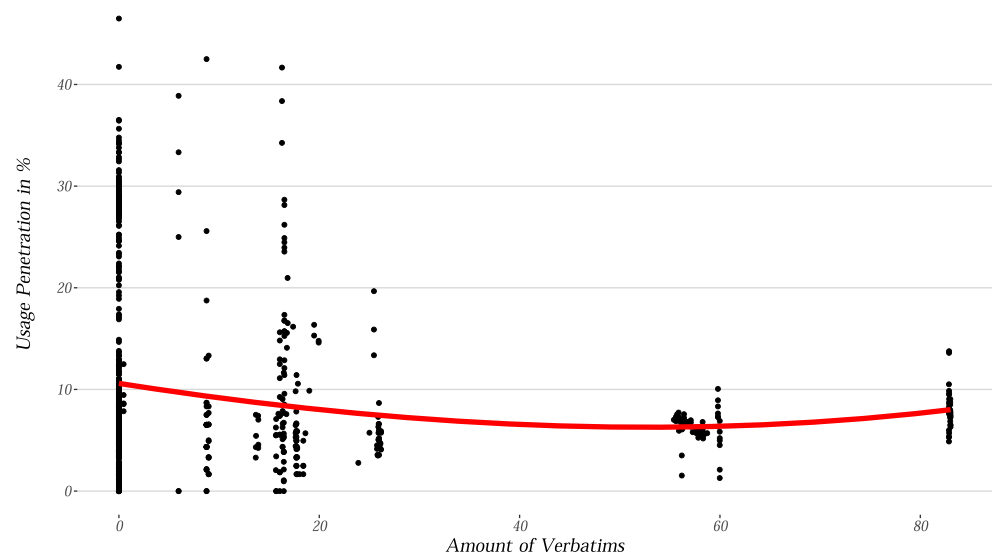
Fig. 10 Usage Penetration Values Conditional on the Amount of Verbatims Available in a Client's Software Including Smoothing (Red Line)
