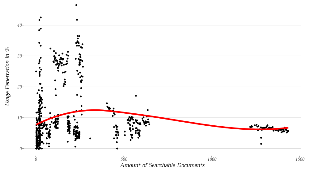
Fig. 12 Usage Penetration Values Conditional on the Amount of Searchable Documents Available in a Client's Software Including Smoothing (Red Line)
