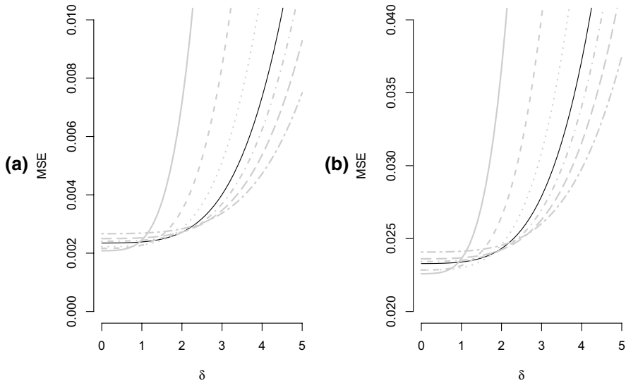
Fig. 2 MSE of \widehat{\sigma^2}_{\text{Mean}} when choosing n = \frac{\sqrt{N}}{K+1} for true K = 3 (—), K = 0 (---) K = 1 (- - -) K = 2 (· · · ·) K = 4 (· · · ·) K = 5 (---) and K = 6 (- - -) with N = 1000 and h = \delta \cdot \sigma , \delta \in \{0, 0.1, \dots, 5\} , Y_t = X_t + \sum_{k=1}^3 hI_{t \geq t_k} , where a X_t \sim N(0, 1) and b X_t \sim t_3
