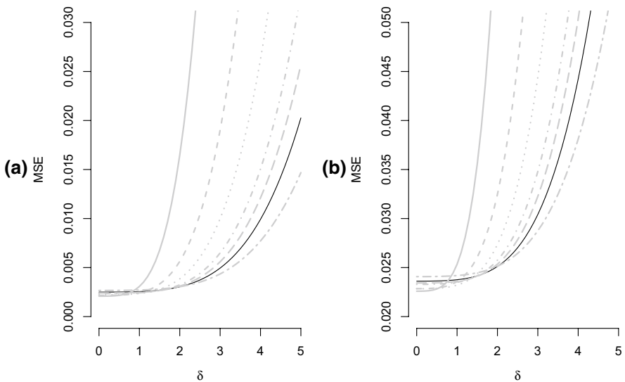
Fig. 8 MSE of \widehat{\sigma}^2_{\text{Mean}} when choosing n = \frac{\sqrt{N}}{K+1} for true K = 5 (—), K = 0 (— — —) K = 1 (- - -) K = 2 (· · · ·) K = 3 (- · · -) K = 4 (- - - -) and K = 6 (- - - -) with N = 1000 and h = \delta \cdot \sigma , \delta \in \{0, 0.1, \dots, 5\} , Y_t = X_t + \sum_{k=1}^5 hI_{\geq t_k} , where a X_t \sim N(0, 1) and b X_t \sim t_3
