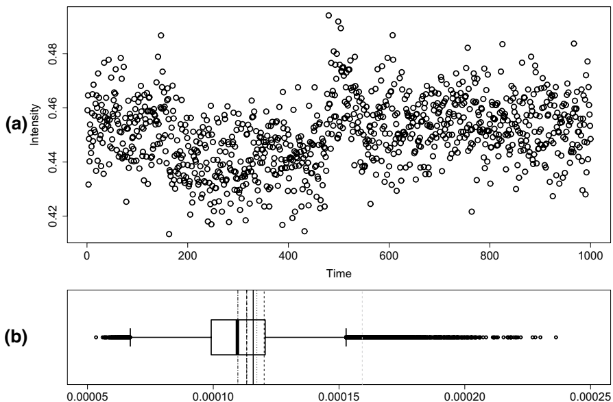
Fig. 5 a Intensity over time for one pixel and b a boxplot of variances for the virus-free pixels together with the ordinary sample variance of the above data (---) and values of \widehat{\sigma}_{\text{Mean}}^2 and \widehat{\sigma}_{\text{Diff}}^2 (—), \widehat{\sigma}_{\text{Tr},0.5}^2 (---), \widehat{\sigma}_{\text{Tr,rad}}^{\text{norm}} (····), \widehat{\sigma}_{\text{Tr,rad}}^{\text{other}} (- · - ·), \widehat{\sigma}_{\text{Mean}}^{\text{mosum}} (---) and \widehat{\sigma}_{\text{W}}^{\text{mosum}} (- - -)
