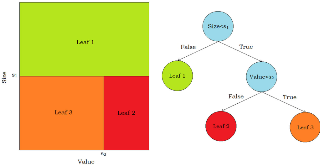
FIGURE 1 Example of regression tree diagram using size and value with L = 2 and regressor space partition into leaves according to splitting points s_1 and s_2 [Colour figure can be viewed at wileyonlinelibrary.com ]
