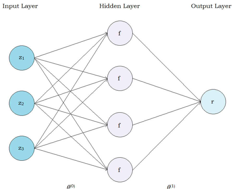
FIGURE 2 Example of FFN with three inputs ( z_1, z_2, z_3 ), one hidden layer with Q = 4 units and activation function f , and output r . Arrows are associated with network weight parameters. [Colour figure can be viewed at wileyonlinelibrary.com ]
