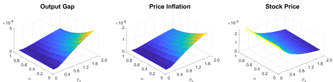
FIGURE 7 Variances of y_t , \pi_t and s_t at different combinations of \phi_s and \kappa , based on a Monte-Carlo simulation of 10,000 runs with \sigma_{\epsilon^\pi} = 0.05 and \sigma_{\epsilon^r} = \sigma_{\epsilon^y} = 0 [Colour figure can be viewed at wileyonlinelibrary.com ]
