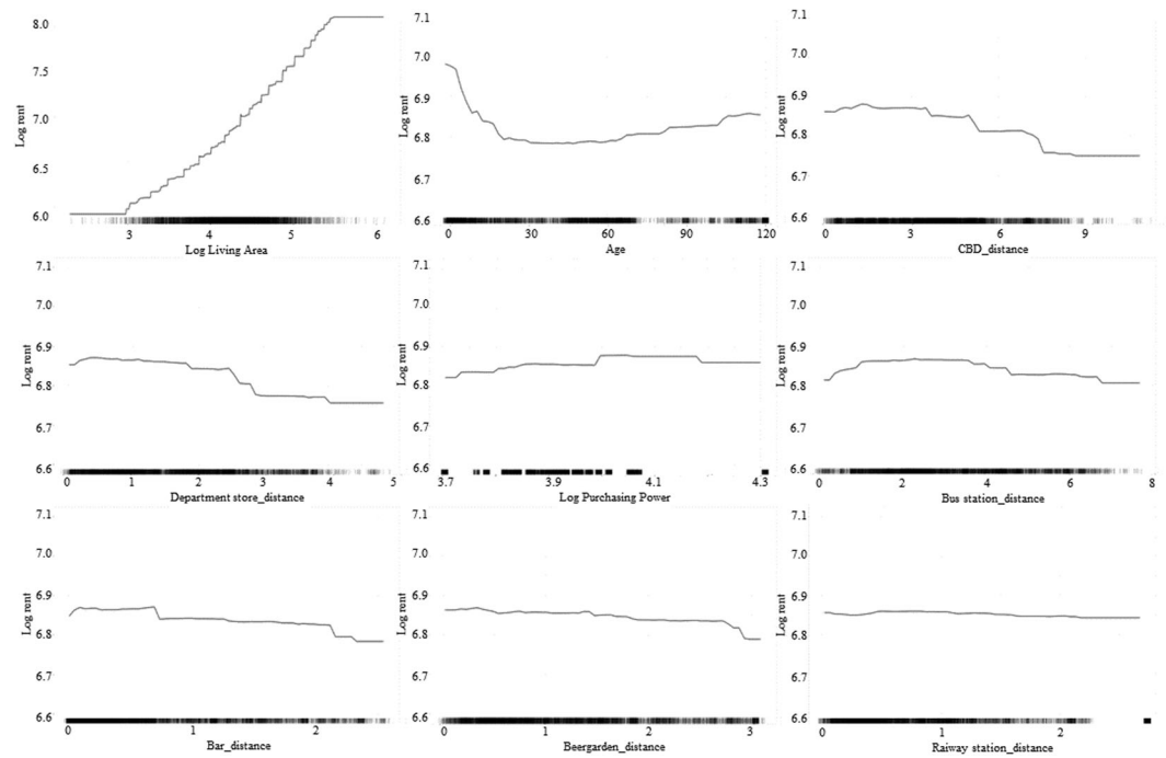
FIGURE 5 First set of PD Plots for the year 2019 Note: The figure displays the partial dependence of size in square meter, age, distance to CBD, department store, bus station, bar, beergarden, railway station, and purchasing power. The vertical axis denotes the feature values of log rent level while the horizontal axis represents the covariates feature values. Stacked black lines display the number of observations. Source: Own depiction.
