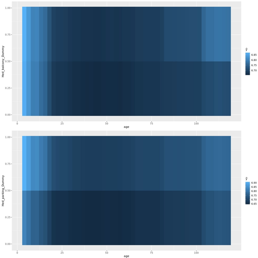
FIGURE 14 Two-dimensional PD Plot of the variables age and balcony/parking [Color figure can be viewed at wileyonlinelibrary.com ]
