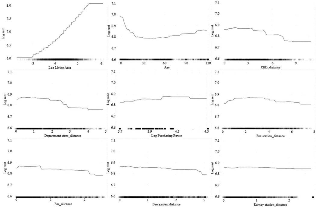
FIGURE 5 First set of PD Plots for the year 2019
