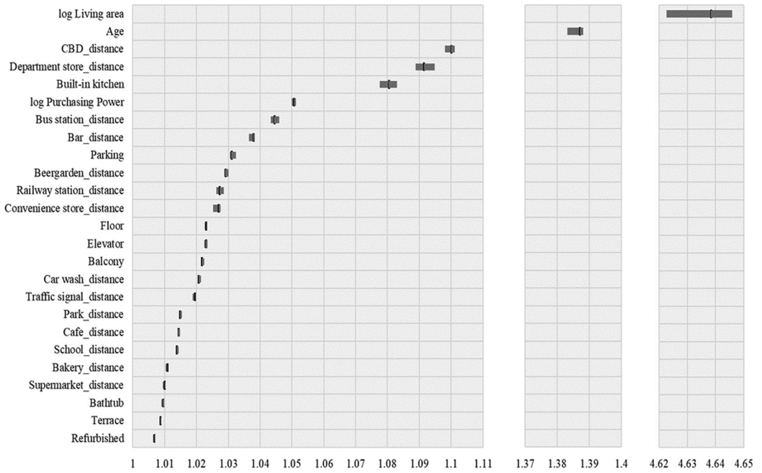
FIGURE 3 Feature importance of the hedonic characteristics
