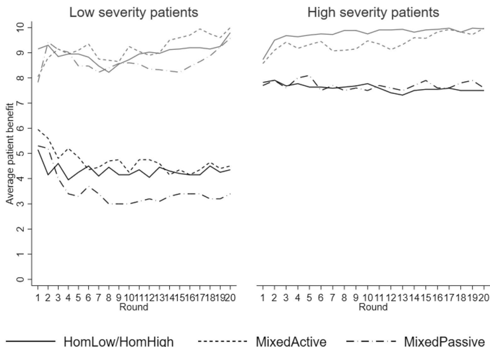
FIGURE 8 Evolution of average benefits for active and passive patients: Evolution of average patient benefit for active (gray line) and passive (black line) patients with competition in HomLow , HomHigh , MixedActive , and MixedPassive . Maximum benefit level resulting from optimal treatment behavior is 10. Minimum benefit level due to physicians' profit maximization is 3 for low-severity patients and 7 for high-severity patients.
