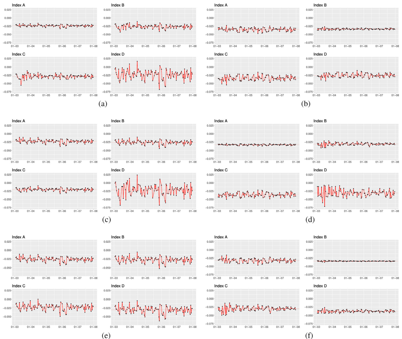
FIGURE 9 Trend of \Delta\text{QL-CoVaR}_{t,\theta,\tau}^{(k)} , with k \in \{A,B,C,D\} clustered by individual pillar. The underlying QL-CoVaR model is estimated using the data observed from March 3, 2020, to July 31, 2020 (a) EU companies—clustered by \bar{\text{E-Pillar}} classes (b) US companies—clustered by \bar{\text{E-Pillar}} classes (c) EU companies clustered by \bar{\text{S-Pillar}} classes (d) US companies clustered by \bar{\text{S-Pillar}} classes (e) EU companies clustered by \bar{\text{G-Pillar}} classes (f) US companies clustered by \bar{\text{G-Pillar}} classes [Colour figure can be viewed at wileyonlinelibrary.com ]
