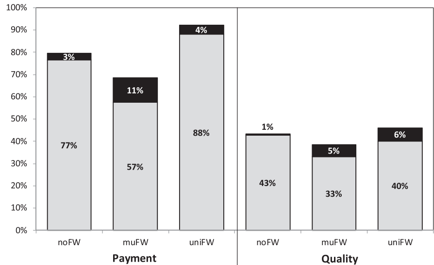
FIGURE 1 Average payment/revenues and quality/efficiency conditional on trade, across the three treatments. The figure reports initial payment and quality in the transaction stage (gray share of the bars), as well as additionally provided payments and quality in the make-good stage (black share of the bars). Numbers are based on rounds 11–50 in the experiment.
