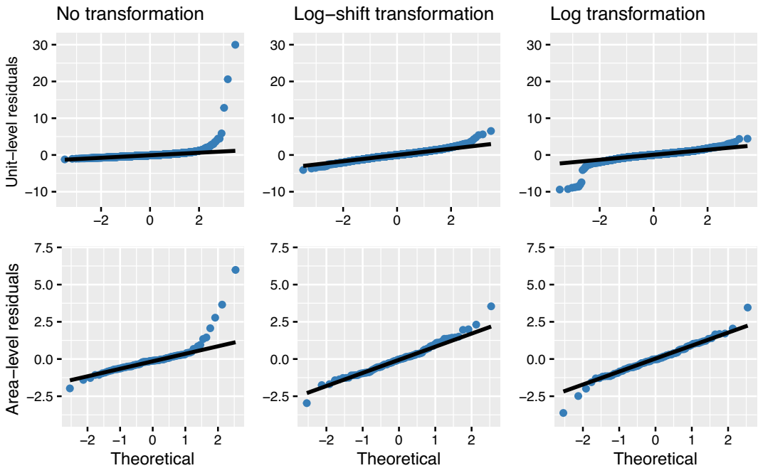
FIGURE 2 QQ-plots for the individual-level residuals (first row) and the area-level residuals (second row) among the nested error regression models under different transformations. [Colour figure can be viewed at wileyonlinelibrary.com ]
