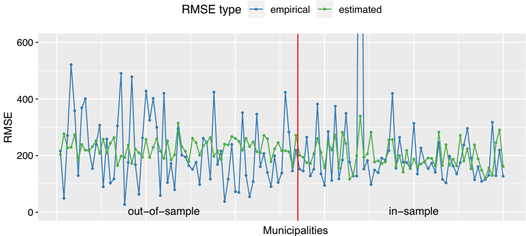
FIGURE 5 Estimated and empirical municipal-specific root mean squared error using the proposed estimator (10) with log-shift transformation in design-based simulation study. [Colour figure can be viewed at wileyonlinelibrary.com ]
