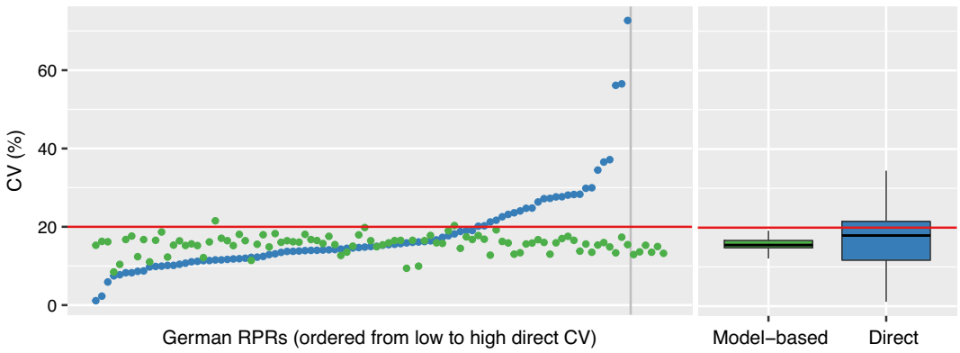
FIGURE 6 Area-specific coefficients of variation (CVs) for the direct (blue) and the proposed model-based (green) estimates, ordered from low to high CVs for direct estimates and the associated boxplots. The grey line in the left plot separates the non-sampled areas. The red line marks the 20%-threshold for defining reliable estimates. [Colour figure can be viewed at wileyonlinelibrary.com ]
