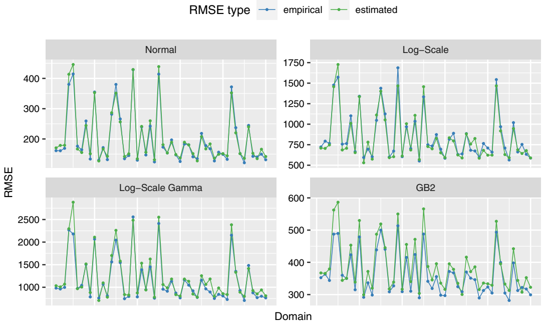
FIGURE 4 Estimated and empirical domain-specific root mean square errors using the proposed estimator (10) with log-shift transformation in model-based simulations. [Colour figure can be viewed at wileyonlinelibrary.com ]
