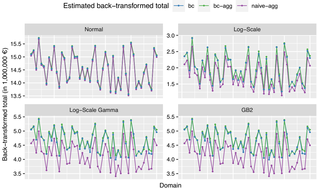
FIGURE 3 Estimated back-transformed totals bc \left( T_i = \sum_{j=1}^{N_i} \exp(x_j^T \hat{\beta}) \right) , bc\text{-agg} \left( \hat{T}_i \right) and naive\text{-agg} \left( \exp \left( \bar{x}_i^T \hat{\beta} \right) \right) over the domains for one arbitrarily chosen Monte-Carlo simulation. [Colour figure can be viewed at wileyonlinelibrary.com ]
