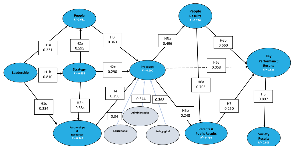
Figure 1. The research model and the direct effects after applying PLS algorithm.
