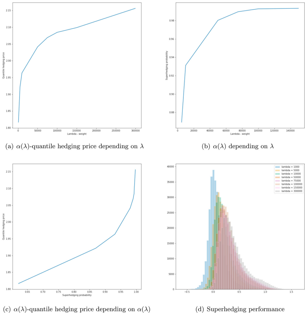
FIGURE 3 Impact of \lambda on the quantile hedging price and on the superhedging probability for l = (\max\{\frac{1}{1+e^{-x}} - \frac{1}{2}, 0\})^2 [Color figure can be viewed at wileyonlinelibrary.com ]
