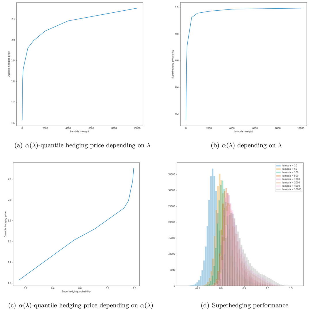
FIGURE 2 Impact of \lambda on the quantile hedging price and on the superhedging probability for l = (\max\{x, 0\})^2 [Color figure can be viewed at wileyonlinelibrary.com ]
