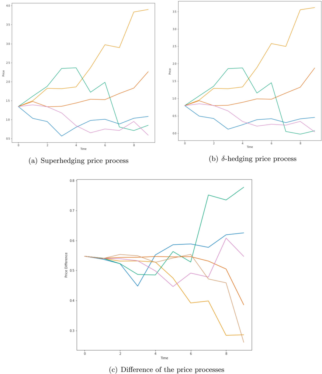
FIGURE 5 Superhedging price process compared to the \delta -hedging price process [Color figure can be viewed at wileyonlinelibrary.com ]
