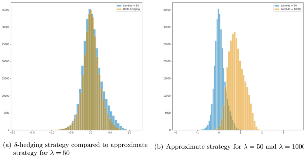
FIGURE 4 Hedging losses for \lambda = 50 , \lambda = 10000 and for the \delta -hedging strategy [Color figure can be viewed at wileyonlinelibrary.com ]
