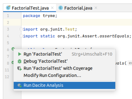
Figure 14: Exemplary screenshot of the run line marker in IntelliJ to start the dynamic analysis for Dacite.
