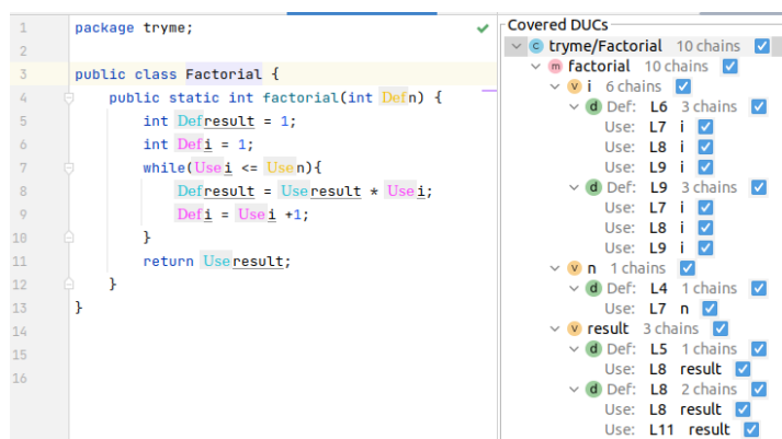
Figure 1: Exemplary screenshot of the Dacite visualization in IntelliJ based on given test.
