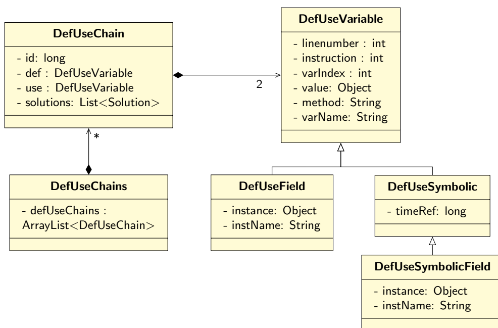
Figure 7: An overview of the DUCs implementation in the package analysis. Methods are omitted for the sake of clarity [22].
