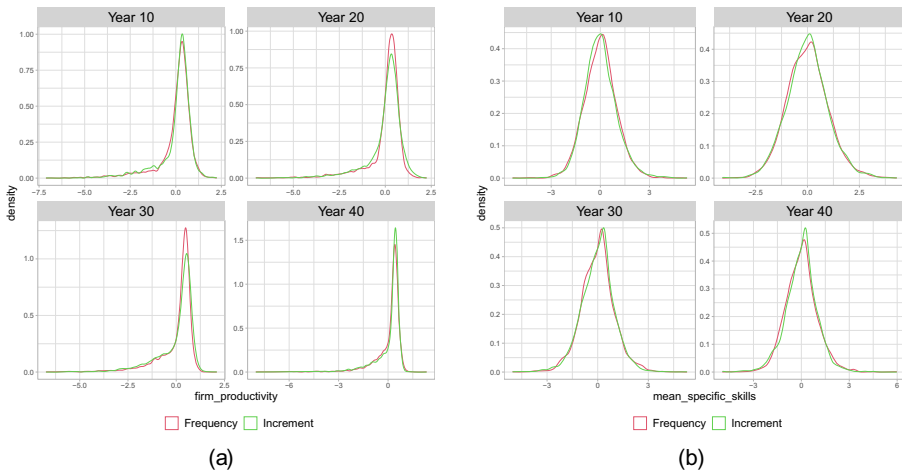
Fig. 7 Standardized distribution of firm productivity (a) and specific skills (b) , pooled over 40 Monte Carlo simulations with homogeneous general skills, for years 10, 20, 30, 40 after the shift in the technological regime
