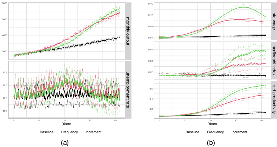
Fig. 2 Aggregate dynamics. (a) (1) Aggregate output (top) and (2) unemployment (bottom). (b) (1) standard deviation for wages (top), (2) Herfindahl index (middle) and (3) standard deviation in firm productivity (bottom)
