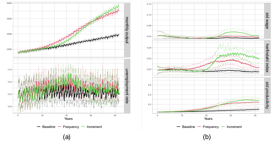
Fig. 6 Aggregate dynamics under homogeneous general skills. (a) (1) Aggregate output (top) and (2) unemployment (bottom). (b) (1) standard deviation for wages (top), (2) Herfindahl index (middle) and (3) standard deviation in firm productivity (bottom)
