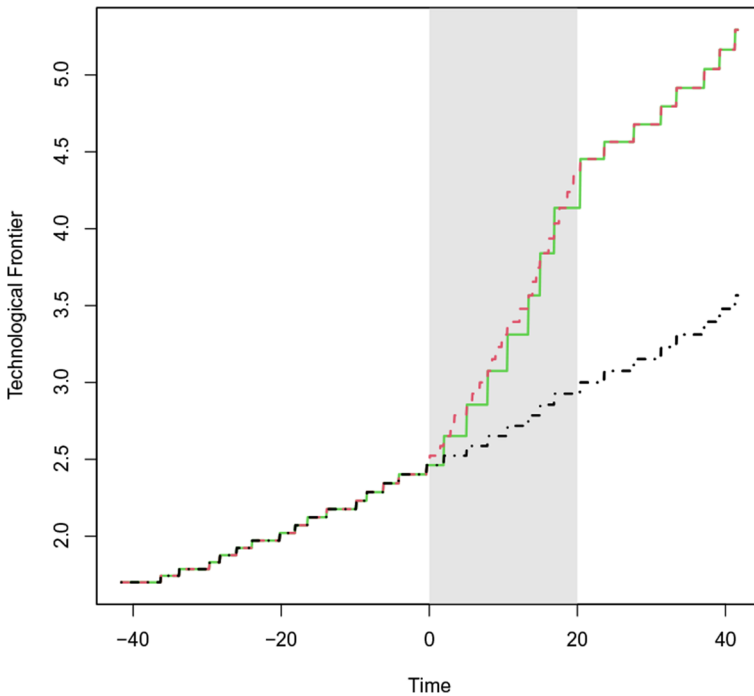
Fig. 1 Technological frontier A^V_t (the most productive vintage in time t ). Grey area indicates the regime shift. Baseline in black, Frequency in red and Increment in green
