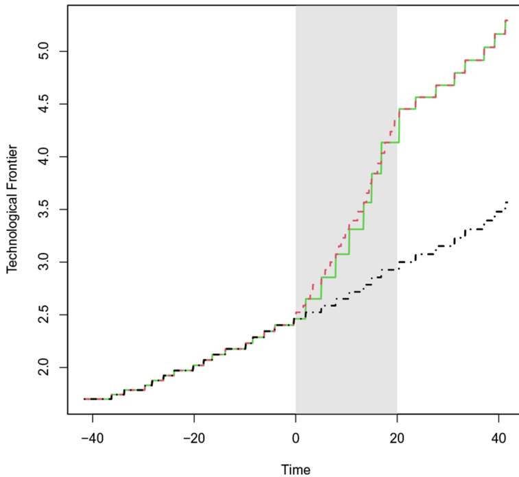
Fig. 1 Technological frontier A_t^V (the most productive vintage in time t ). Grey area indicates the regime shift. Baseline in black, Frequency in red and Increment in green
