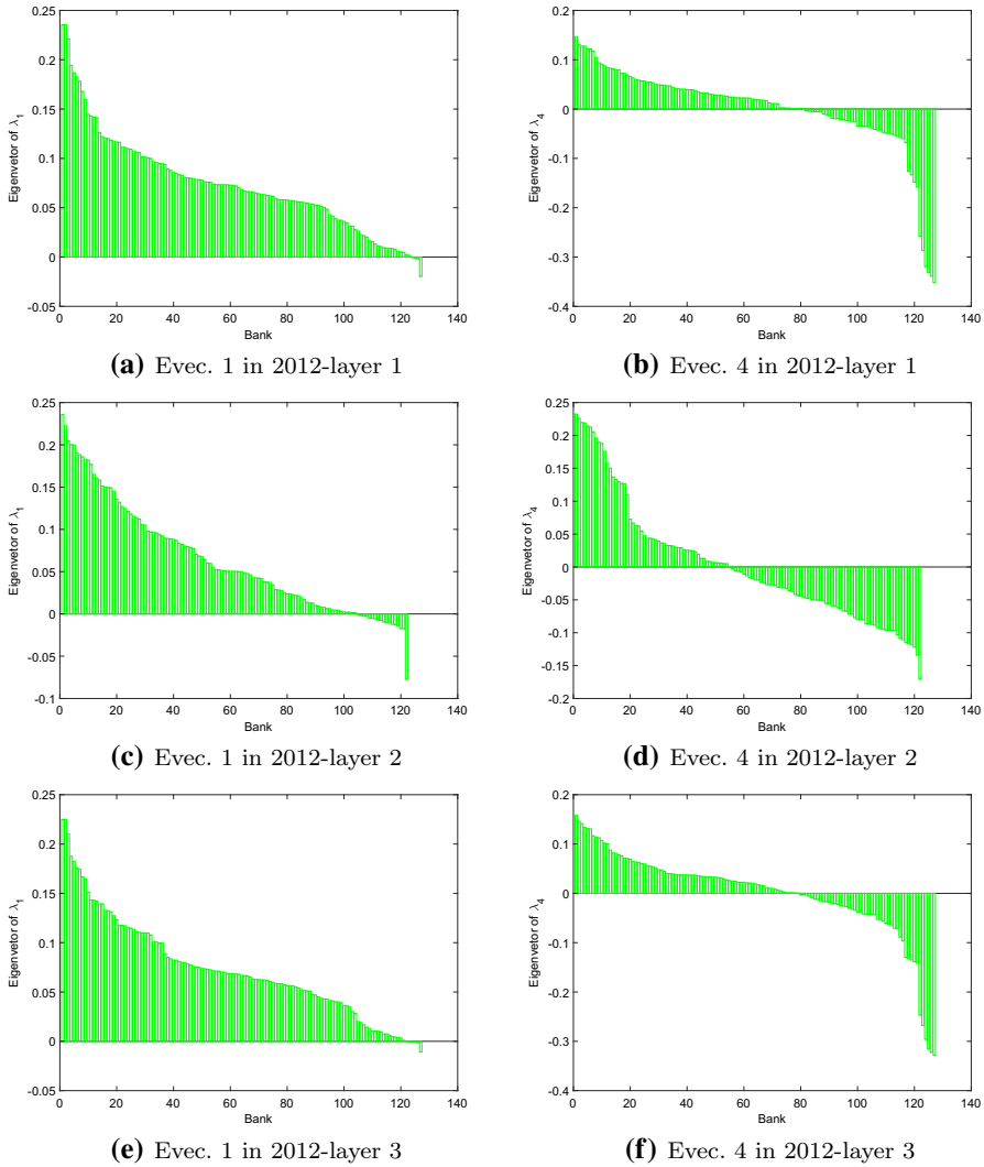
Fig. 13 The eigenvectors (sorted in descending order) of \lambda_1 and \lambda_4 , in the three layers, in 2012. Without loss of generality, we fix the signs of eigenvector elements such that their sum is non-negative. Panels a, b show the eigenvectors of \lambda_1 and \lambda_4 in the layer 1. Panels c, d show the eigenvectors of \lambda_1 and \lambda_4 in the layer 2. Panels e, f show the eigenvectors of \lambda_1 and \lambda_4 in the layer 3
