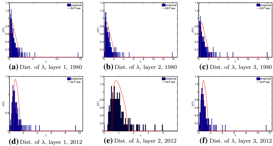
Fig. 19 Binary data: Distribution of eigenvalues of C^{bin} , compared with RMT, in the three layers, in 1980 and 2012. Panels a–c show the distributions of \lambda in 1980, and panels d–f show the distributions of \lambda in 2012. In all panels, the red curve represents the spectral distribution explained by the Marchenko-Pastur law. (Colour figure online)
