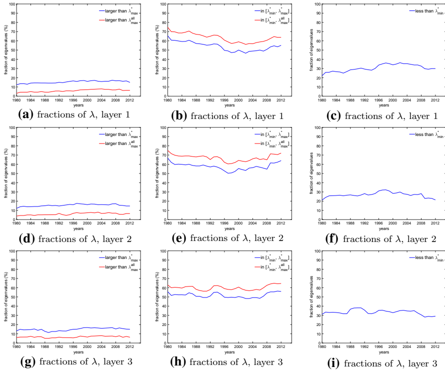
Fig. 11 Fractions of eigenvalues in different ranges for the three layers. Panels a, d, g Fractions of eigenvalues larger than the considered upper bound \lambda_{max}^* (blue lines) or \lambda_{max}^{all} (red lines) for layers 1, 2, 3, respectively. Panels b, e, h Fractions of eigenvalues lie within [\lambda_{min}^*, \lambda_{max}^*] (blue lines) or [\lambda_{min}^*, \lambda_{max}^{all}] (red lines) for layers 1, 2, 3, respectively. Panels c, f, i Fractions of eigenvalues less than the lower bound \lambda_{min}^* for layers 1, 2, 3, respectively. (Colour figure online)
