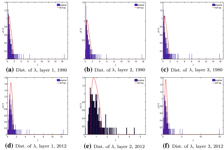
Fig. 3 Distributions of the eigenvalues of the correlation matrices, compared with RMT, in the three layers, in 1980 and 2012. Panels a–c show the distributions of \lambda in 1980, and d–f show the distributions of \lambda in 2012. In all panels, the red curve represents the spectral distribution explained by the Marchenko-Pastur law. Note that over the years, we observe that the top five largest eigenvalues of the empirical correlation matrix in each lending layer are always larger than the three upper bounds \lambda_{max}^* , \lambda_{max}^{(1)} and \lambda_{max}^{(2)} (see also Fig. 11 in the “Appendix”)
