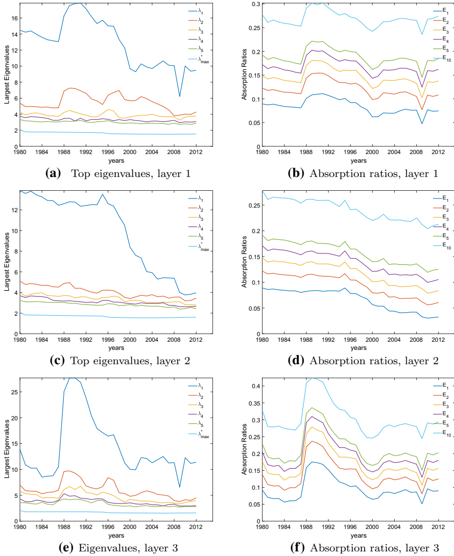
Fig. 20 Binary data: Evolution of the top 5 largest eigenvalues and the associated absorption ratios for C^{bin} in the three layers. The panels on the left show the evolution of the top 5 largest eigenvalues. These eigenvalues are always larger than the upper bound \lambda_{max}^* implied by RMT. The three panels on the right show their associated absorption ratios as well as the absorption ratio of the top 10 largest eigenvalues
