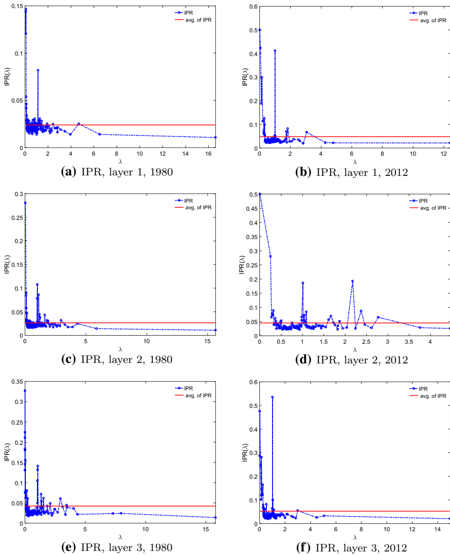
Fig. 5 Inverse Participation Ratios of the eigenvectors of the correlation matrices in the three layers. Panels a, b show IPR versus \lambda in the layer 1, in 1980 and 2012. Panels c, d show IPR versus \lambda in the layer 2, in 1980 and 2012. Panels e, f show IPR versus \lambda in the layer 3, in 1980 and 2012. The red lines stand for the averages of \{IPR_k\}_{k=1}^{k=N}
