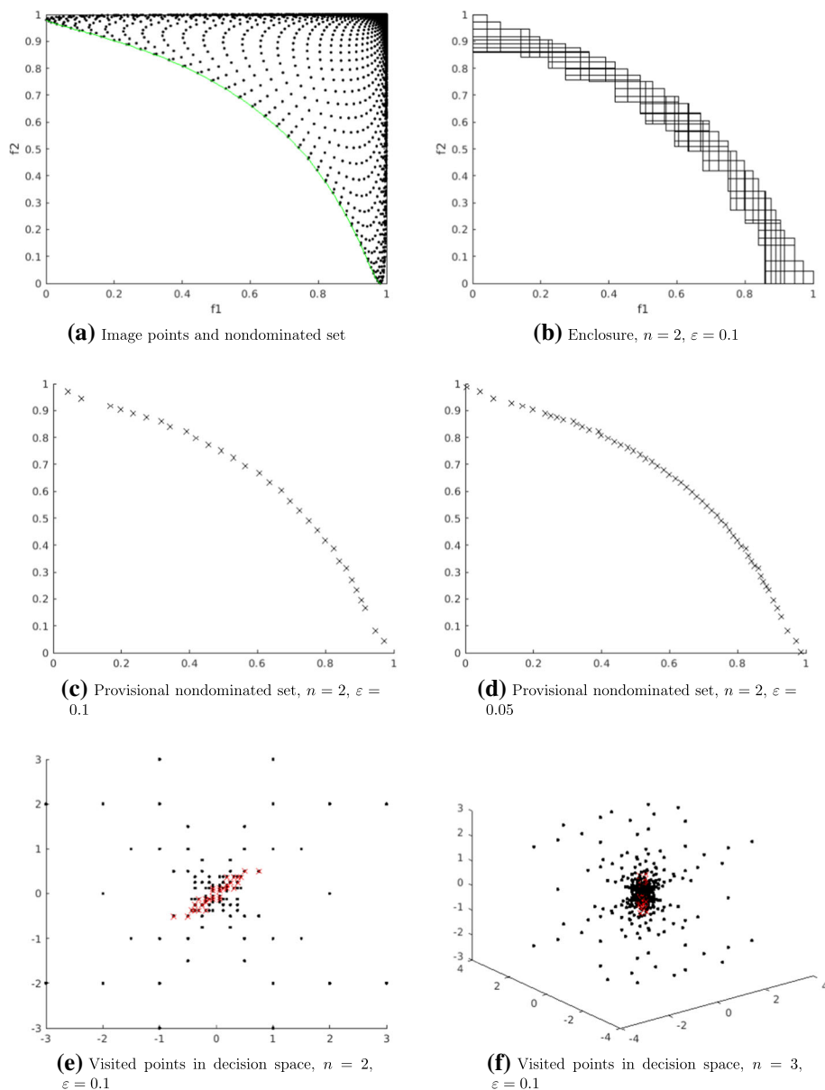
Fig. 2 Test problem FF (Fonseca–Fleming)
