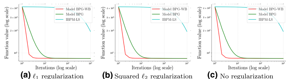
Fig. 3 In this experiment we compare the performance of Model BPG, Model BPG with Backtracking (denoted as Model BPG-WB) and IBPM-LS [45] on Poisson linear inverse problems with \ell_1 regularization, squared \ell_2 regularization and with no regularization. We set the regularization parameter \lambda to 0.1. The plots illustrate that Model BPG-WB is faster in all the settings, followed by Model BPG
