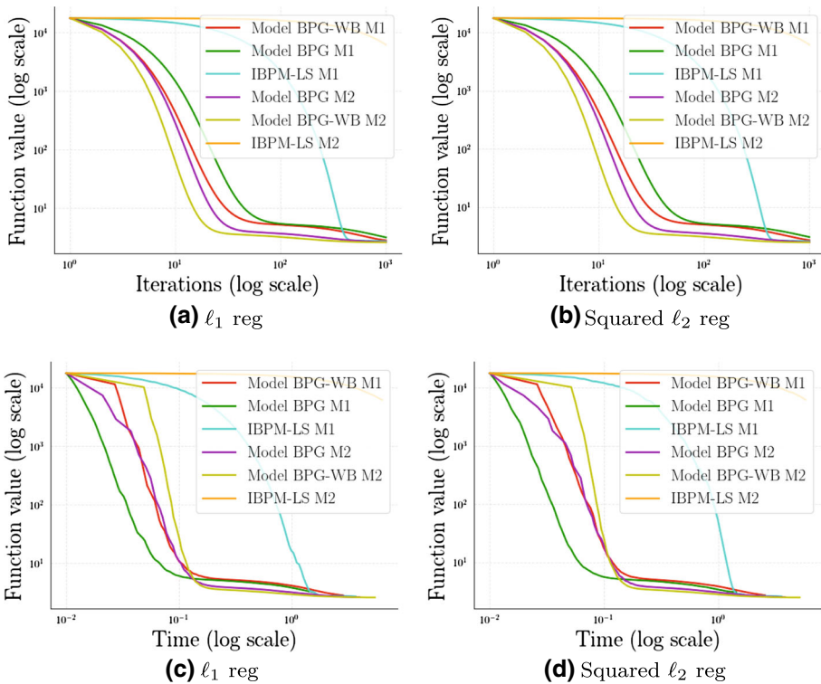
Fig. 1 In this experiment we compare the performance of Model BPG, Model BPG with Backtracking (denoted as Model BPG-WB), and IBPM-LS [45] on standard phase retrieval problems, with both \ell_1 and squared \ell_2 regularization. For this purpose, we consider M1 model function as in (41) without absolute sign (which is the same setting as Bolte et al. [16]), and with M2 model function as in (44). Model BPG with M2 (44) is faster in both the settings and Model BPG variants perform significantly better than IBPM-LS. By reg , we mean regularization
