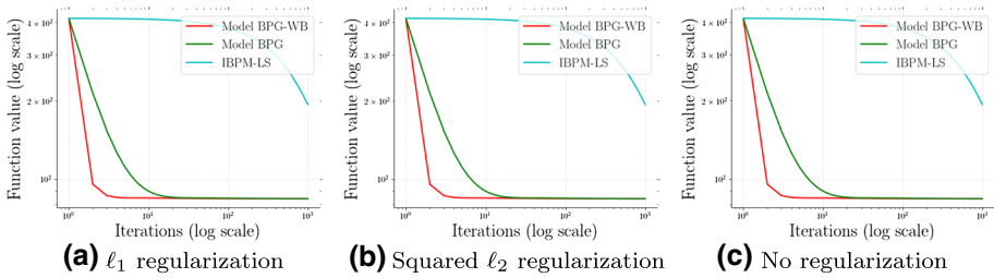
Fig. 3 In this experiment we compare the performance of Model BPG, Model BPG with Backtracking (denoted as Model BPG-WB) and IBPM-LS [45] on Poisson linear inverse problems with \ell_1 regularization, squared \ell_2 regularization and with no regularization. We set the regularization parameter \lambda to 0.1. The plots illustrate that Model BPG-WB is faster in all the settings, followed by Model BPG
