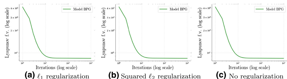
Fig. 4 Under the same setting as in Fig. 3, we illustrate here that Model BPG results in sequences that have monotonically nonincreasing Lyapunov function value evaluations. By Lyapunov f.v. we mean Lyapunov function values
