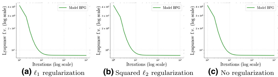
Fig. 4 Under the same setting as in Fig. 3, we illustrate here that Model BPG results in sequences that have monotonically nonincreasing Lyapunov function value evaluations. By Lyapunov f.v. we mean Lyapunov function values
