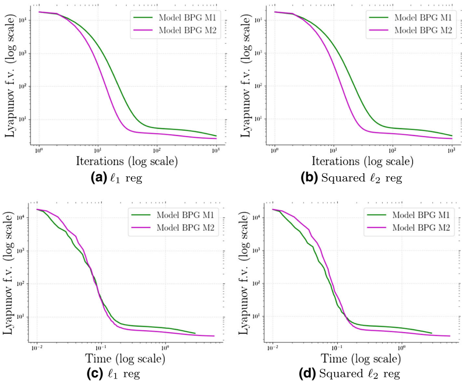
Fig. 2 We illustrate that when Model BPG applied to standard phase retrieval problem in (40), with model function chosen to be either Model 1 in (41) or Model 2 in (44), result in sequences where the Lyapunov function value evaluations are monotonically nonincreasing. In terms of iterations, Model BPG with Model 2 (Model BPG M2) is better than Model BPG with Model 1 (Model BPG M1). In terms of time, Model BPG M1 and Model BPG M2 perform almost the same, however, towards the end Model BPG M2 is faster in both the cases. By reg we mean regularization , and by Lyapunov f.v. we mean Lyapunov function values
