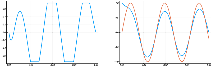
Fig. 1 (l) Optimal solution z_{\mathbb{P}} of (25) for M = 100, h = 1/(2^{10} - 1) . (r) Empirical mean value of u(z_{\mathbb{P}}) out of sample using 1000 iid random realizations of (\xi_1, \dots, \xi_4)
