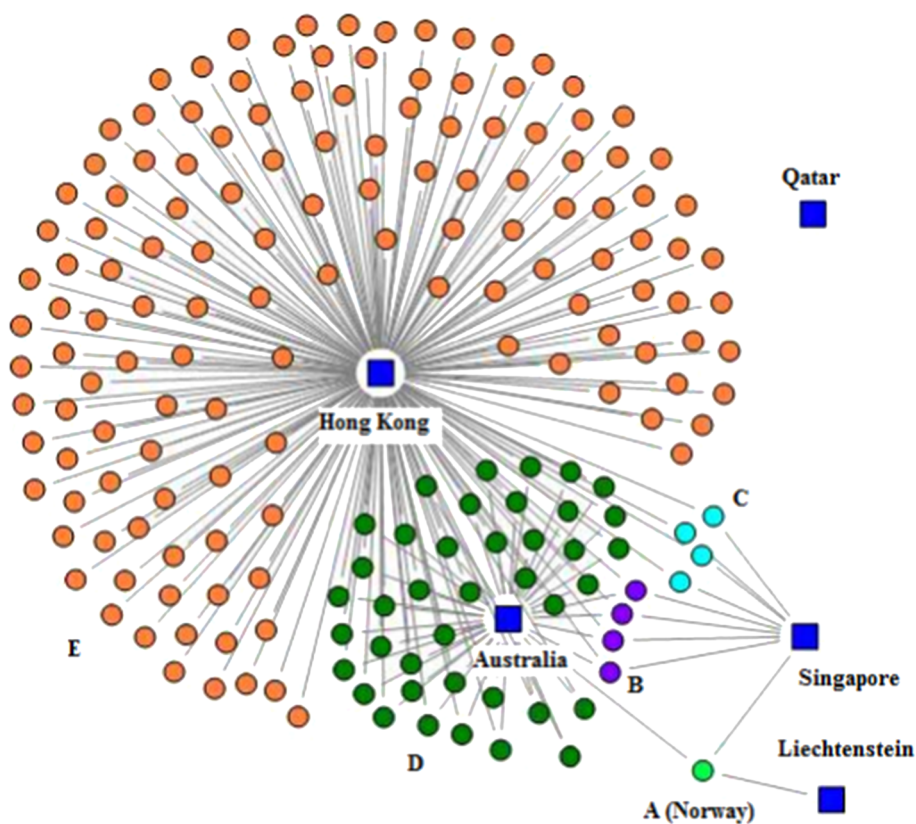
Fig. 1 Network of the traditional BoD with raw data
