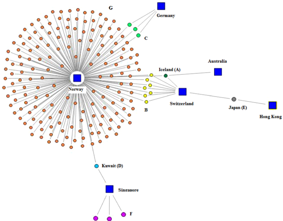
Fig. 5 Network of the SBM-BoD with normalized data
