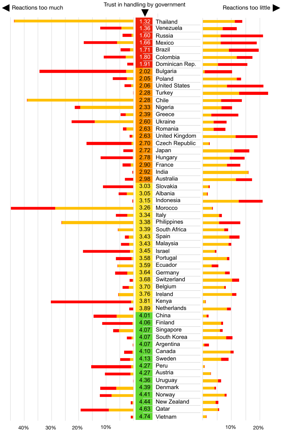
Fig. 1 Perceptions of governments by participants from the respective countries, sorted by government trust (from 1 =“strongly distrust” to 5 =“strongly trust”) based on the survey by Fetzer et al. (2020b). Red = reaction much too extreme/not at all sufficient; orange = somewhat too extreme/somewhat insufficient. (Color figure online)
