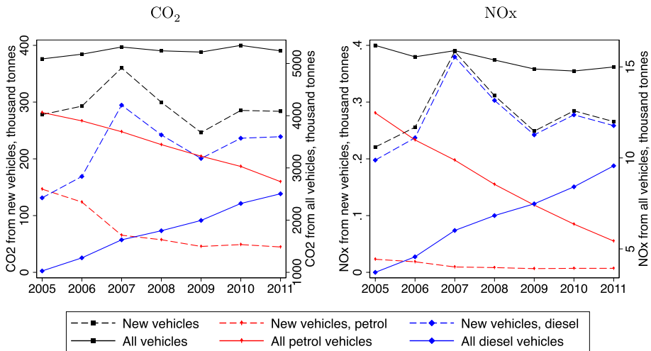
Fig. 4 CO 2 and NOx emissions from passenger cars, by fuel. Note: The two graphs show total CO 2 (in the left panel) and NOx (right panel) emissions from new vehicles (dashed lines) and from all vehicles, by fuel. All emissions are expressed in thousand tonnes. We compute total missions from new vehicles using our data on new registrations. The data source for total emissions from all vehicles is SSB Table 08940 Greenhouses gases, by source (activity, pollutant, contents, and years)
