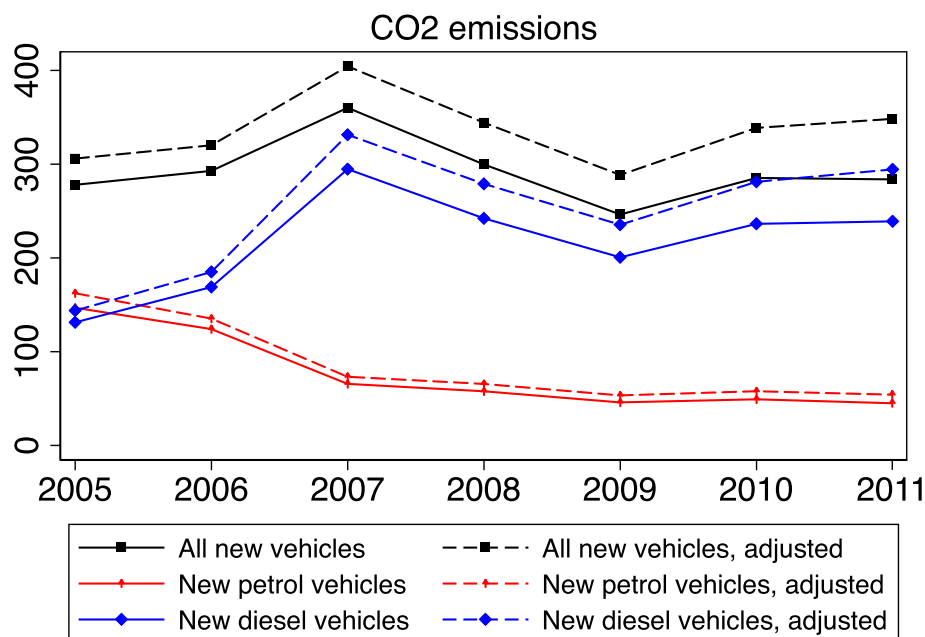
Fig. 14 Total CO 2 emissions from new passenger vehicles, by fuel
