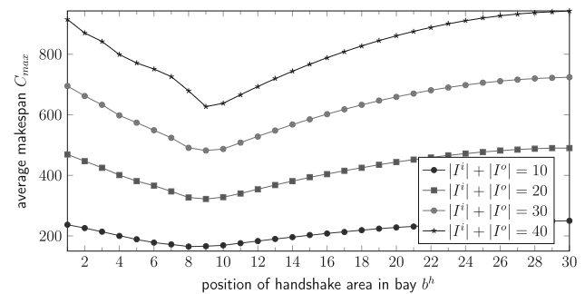
Fig. 4 Average makespan C_{max} for different positions of the handshake area
