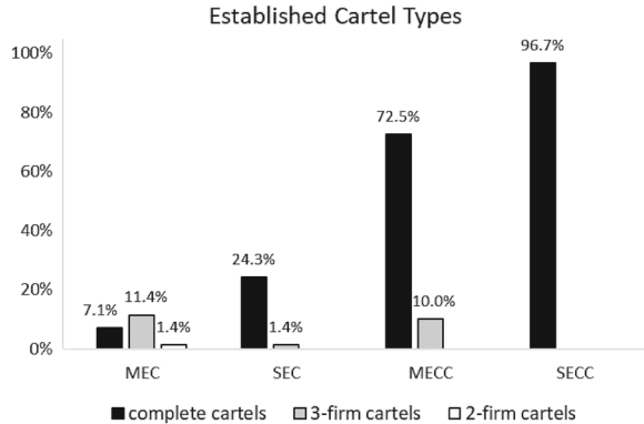
Fig. 1 Percentage of established cartel types
