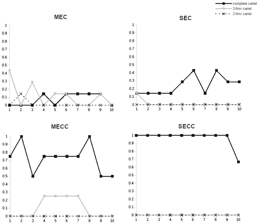
Fig. 2 Percentage of established cartels over time (horizontal axis indicates period number)
