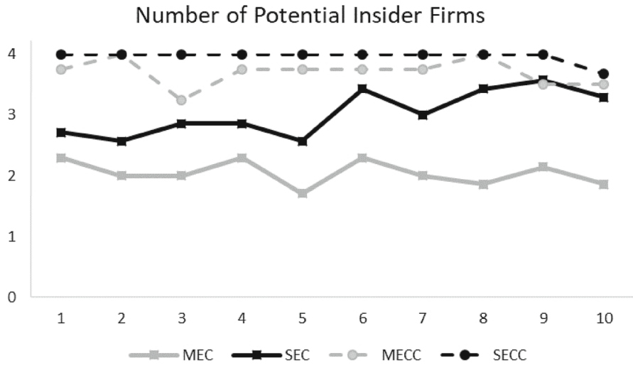
Fig. 3 Number of potential insiders at stage one (horizontal axis indicates period number)
