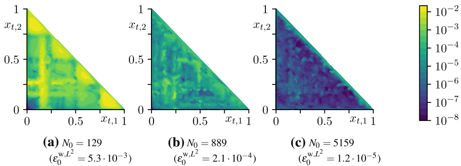
Fig. 10 Pointwise weighted Euler equation error \varepsilon_t^w(x_t) for the two-dimensional transaction costs problem and different spatially adaptive sparse grids at t = 0
