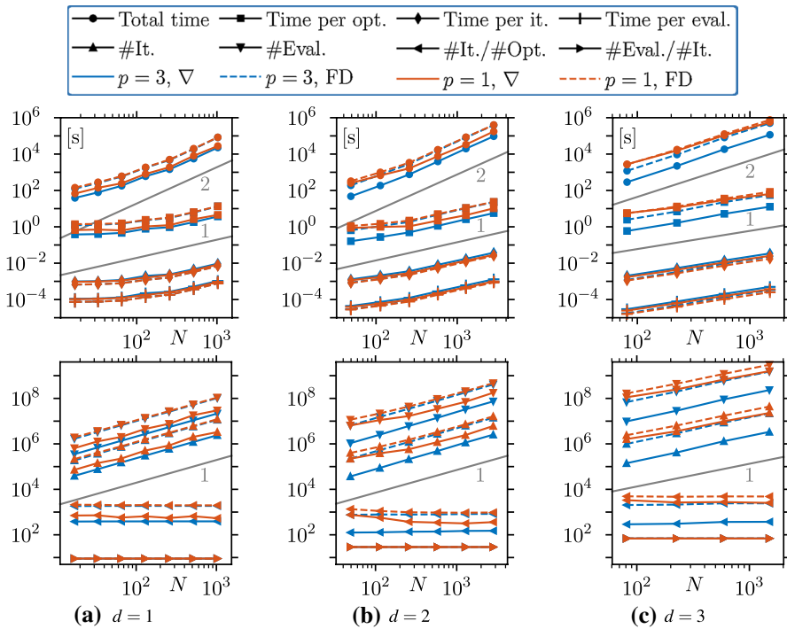
Fig. 8 Computational times (top) and numbers of iterations and evaluations of the interpolant (bottom) for the transaction costs problem on regular sparse grids without refinement. “Total time” is the serial time required to solve all emerging optimization problems. “Time per opt.” is this time divided by the number \#Opt. = TN of optimization problems. “Time per it.” is the total time divided by the number \#It. of optimizer iterations, each of which is assumed to correspond to exactly one combined evaluation of objective function and gradient (the latter only if gradients are used). “Time per eval.” is the total time divided by the number \#Eval. of evaluations of the sparse grid interpolant and its gradient. The colors correspond to B-spline degrees p = 3 or p = 1 and to gradients (“ \nabla ”) or finite differences (“FD”)
