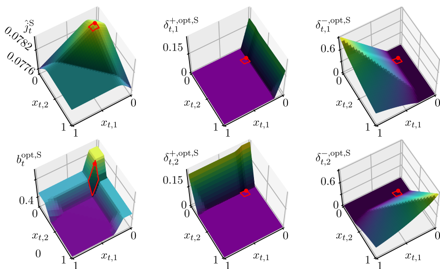
Fig. 7 Full grid solution for the transaction costs problem with d = 2 stocks. Shown are the certainty equivalent value function \hat{J}_t^S(\mathbf{x}_t) (top left) and the optimal policies \mathbf{p}_t^{\text{opt},S}(\mathbf{x}_t) for t = 0 . Also shown are the Merton point \mathbf{x}_t^{\text{opt}} (red dot) and the no-trade region (red outline)
