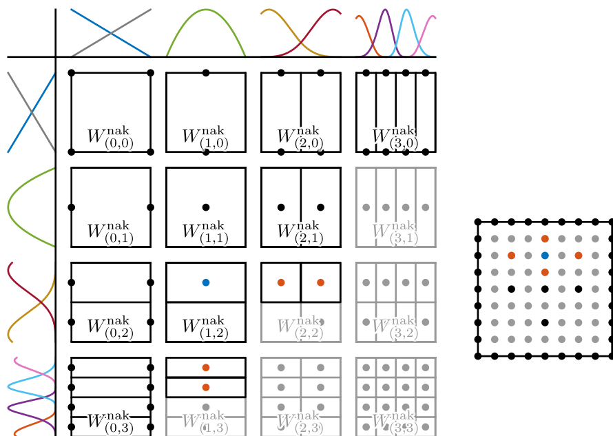
Fig. 4 Spatially adaptive refinement of the hierarchical subspace W_{(1,2)} for the regular sparse grid of level n = 3 in 2D. A refinable grid point (blue) is refined by adding its 2d = 4 children (red). The resulting grid is shown on the right
