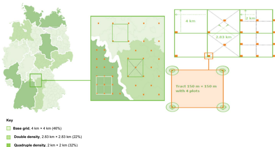
Fig. 2 Germany National Forest grid 2012; source (Polley et al. 2014)
