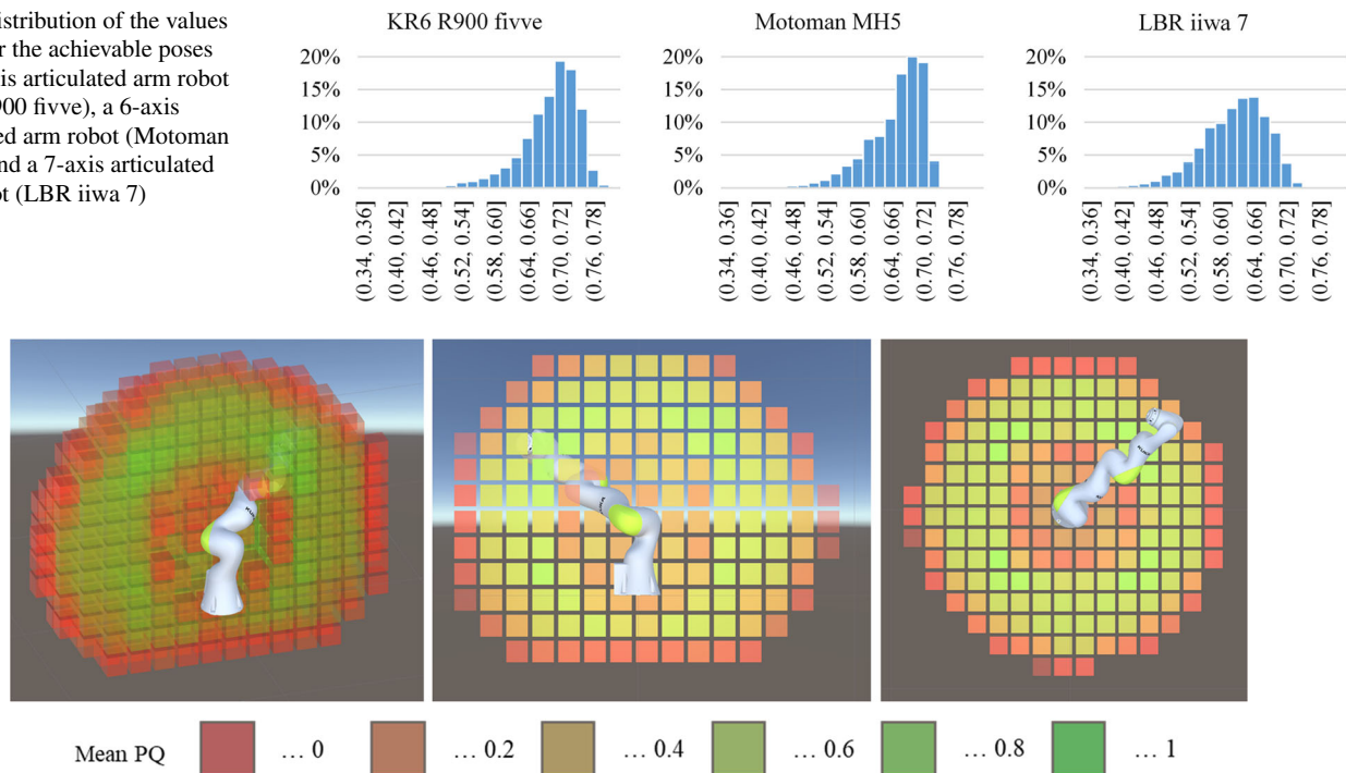
Fig. 7 Examples for the evaluation of positions in the workspace of an LBR iiwa 7 robot, left: 3D view, center: sectional view from left, right: sectional view from above
