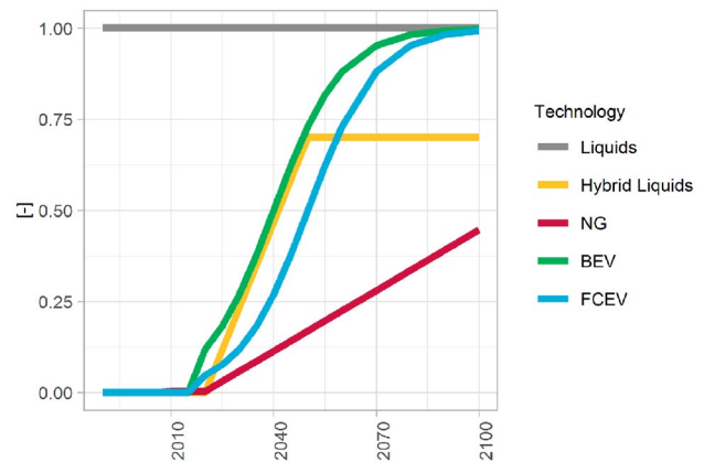
Fig. 8 Preference trend at technology level for Europe, in the illustrative case of LDVs. Consumers equally prefer BEVs and FCEVs by the end of the century. The takeover of hybrid liquids and NG is instead limited
