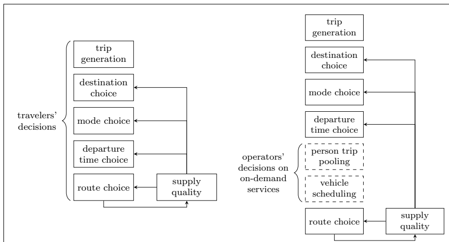
(a) Four-step algorithm supplemented by departure time choice (b) Extended four-step algorithm to model the impact of on-demand services
