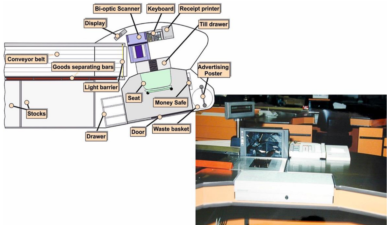
Fig. 31 Schematic layout of the ergonomic scanner checkout with marked components ( upper left part ) and view of the tools used for checking in true perspective of the staff ( lower right part )
