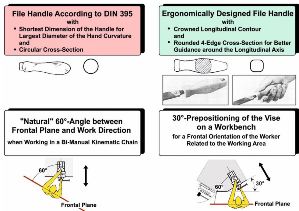
Fig. 26 File handle according to German Standard DIN 395 1968 (upper left part) and an ergonomically designed handle (upper right part), and favorable 30° prepositioning of the vise on a work bench (lower right part)
