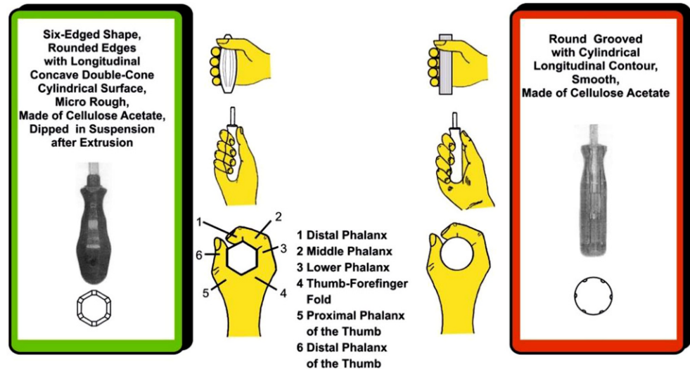
Fig. 21 Screwdriver handle contours, compatible ( left ) and incompatible ( right ) with the hand curvature
