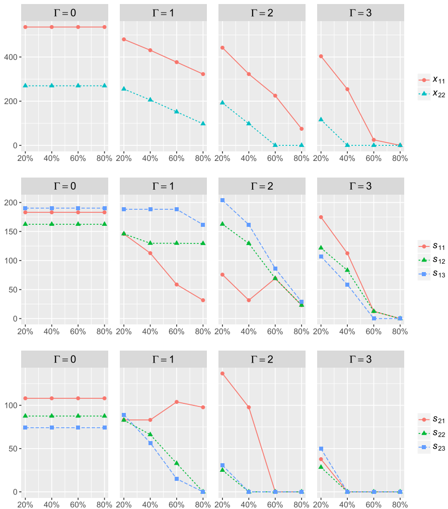
Fig. 3 Top: total generation by each firm ( x_{fi} in MWh). Mid and bottom: Sales by firm 1 (mid; s_{1i} in MWh) and 2 (bottom; s_{2i} in MWh) at each node of the network. All vs. different uncertainty interval sizes and for \Gamma \in \{0, 1, 2, 3\}
