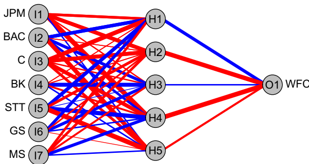
Fig. 3 Fitted quantile regression neural network for Wells Fargo on 13 March 2008. Red connections indicate negative weights, blue connections indicate positive weights
