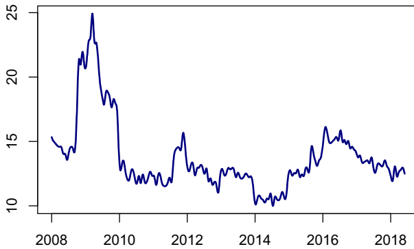
Fig. 6 Time series of the SNRI
