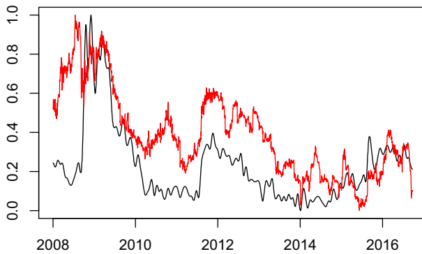
Fig. 8 Co-movement of the SNRI (black line) and the aggregate SRISK (Brownlees and Engle (2017), red line)
