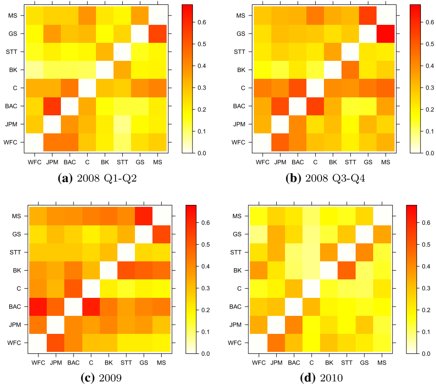
Fig. 4 Time average of risk spillover effects across banks for different time periods
