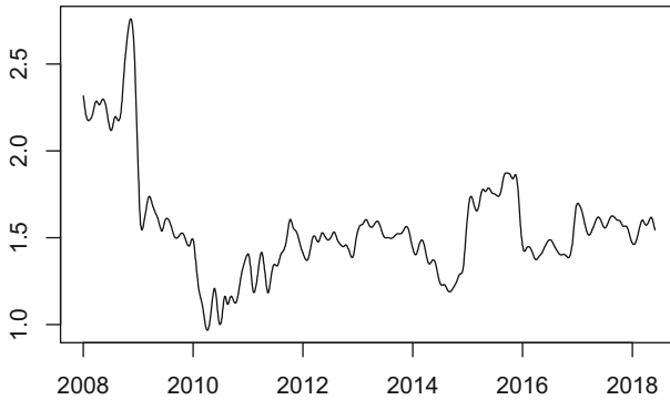
Fig. 9 Time series of the SFI for Citigroup
