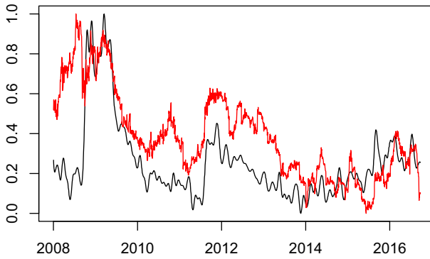
Fig. 12 Co-movement of the SNRI (black line) and the SRISK (Brownlees and Engle (2017), red line), \tau = 1\%
