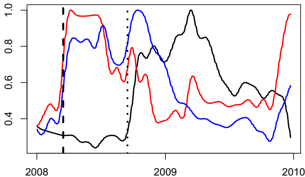
Fig. 7 Plot of SNRI (black line), the Granger causality measure of Billio et al. (2012) (red line) and total connectedness of Diebold and Yılmaz (2014) (blue line). Dashed vertical line marks the bailout and acquisition of Bear Stearns by JP Morgan on 14 March 2008, the dotted vertical line indicates the bankruptcy of Lehman Brothers on 15 September 2008
